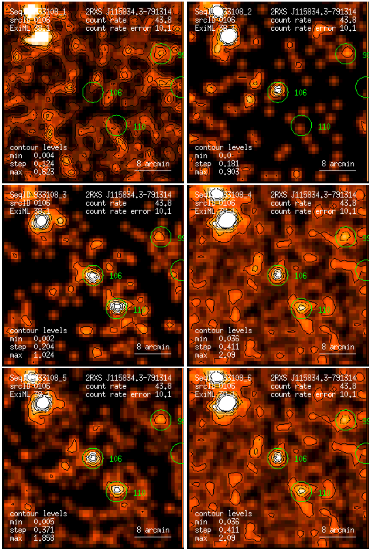
Figure 106: RASS 933108: detection 0106: band rate images, Gaussian filter: (1) PSPC channels 11 – 41, (2) 52 – 90, (3) 91 – 201, (4) 11 – 235, (5) 52 – 201, (6) 11 – 201. Broad band rates in counts/ks. Band rate contour levels in counts/ks/arcmin 2 .
