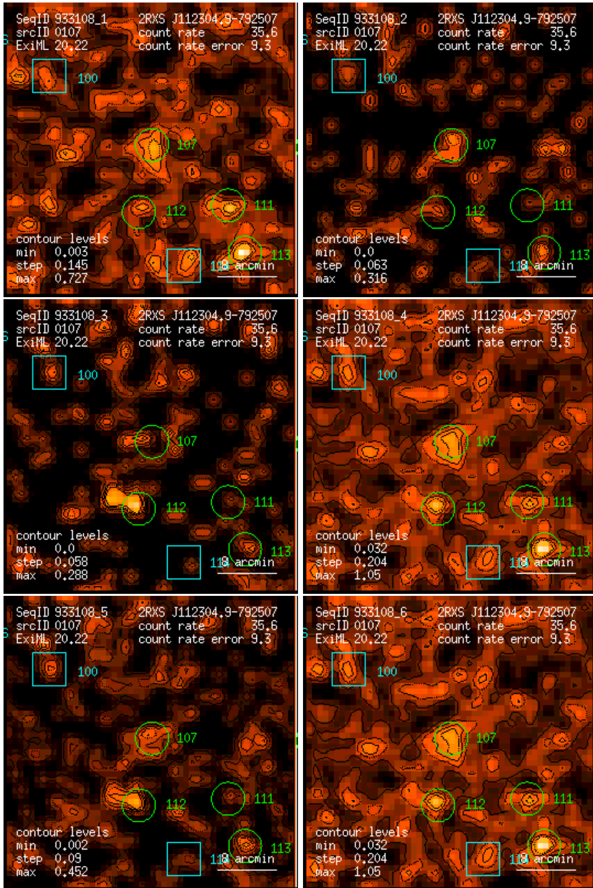
Figure 107: RASS 933108: detection 0107: band rate images, Gaussian filter: (1) PSPC channels 11 – 41, (2) 52 – 90, (3) 91 – 201, (4) 11 – 235, (5) 52 – 201, (6) 11 – 201. Broad band rates in counts/ks. Band rate contour levels in counts/ks/arcmin 2 .
