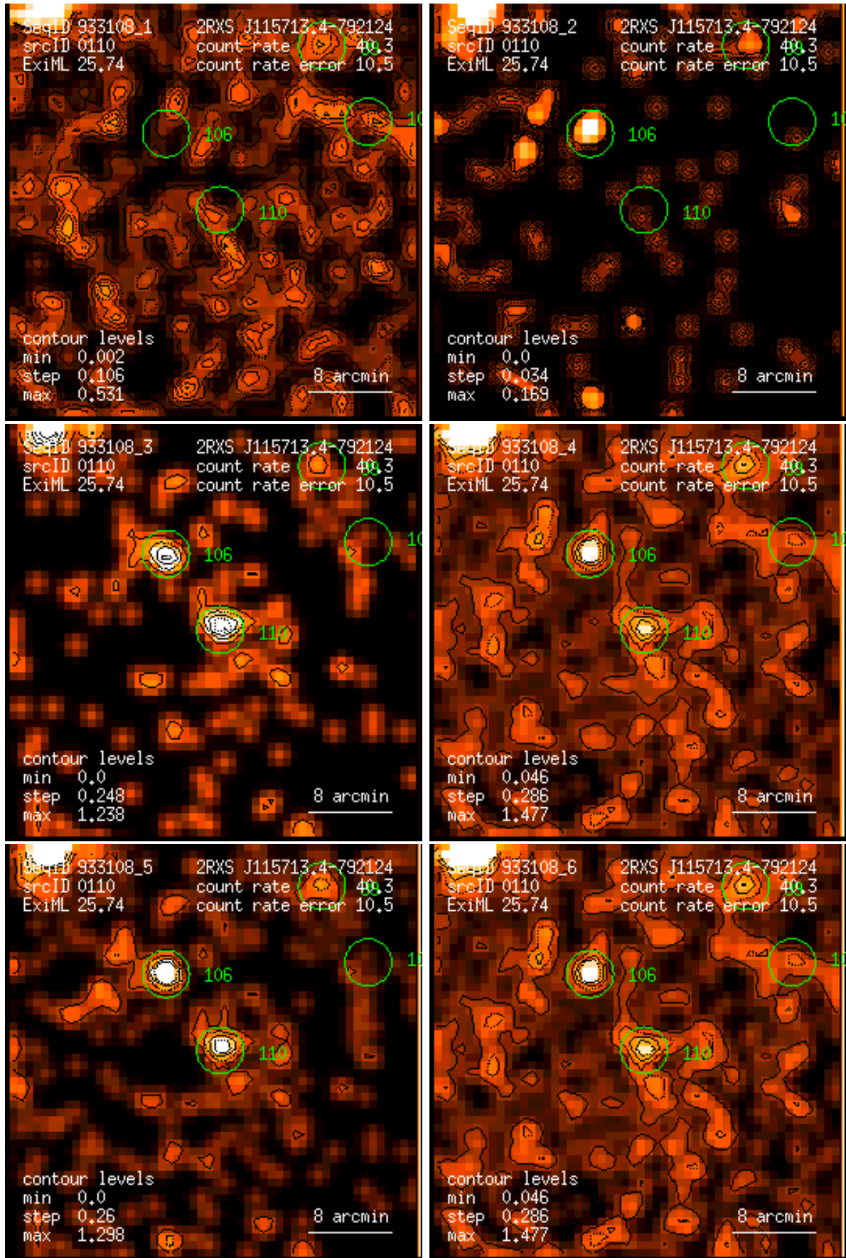
Figure 110: RASS 933108: detection 0110: band rate images, Gaussian filter: (1) PSPC channels 11 – 41, (2) 52 – 90, (3) 91 – 201, (4) 11 – 235, (5) 52 – 201, (6) 11 – 201. Broad band rates in counts/ks. Band rate contour levels in counts/ks/arcmin 2 .
