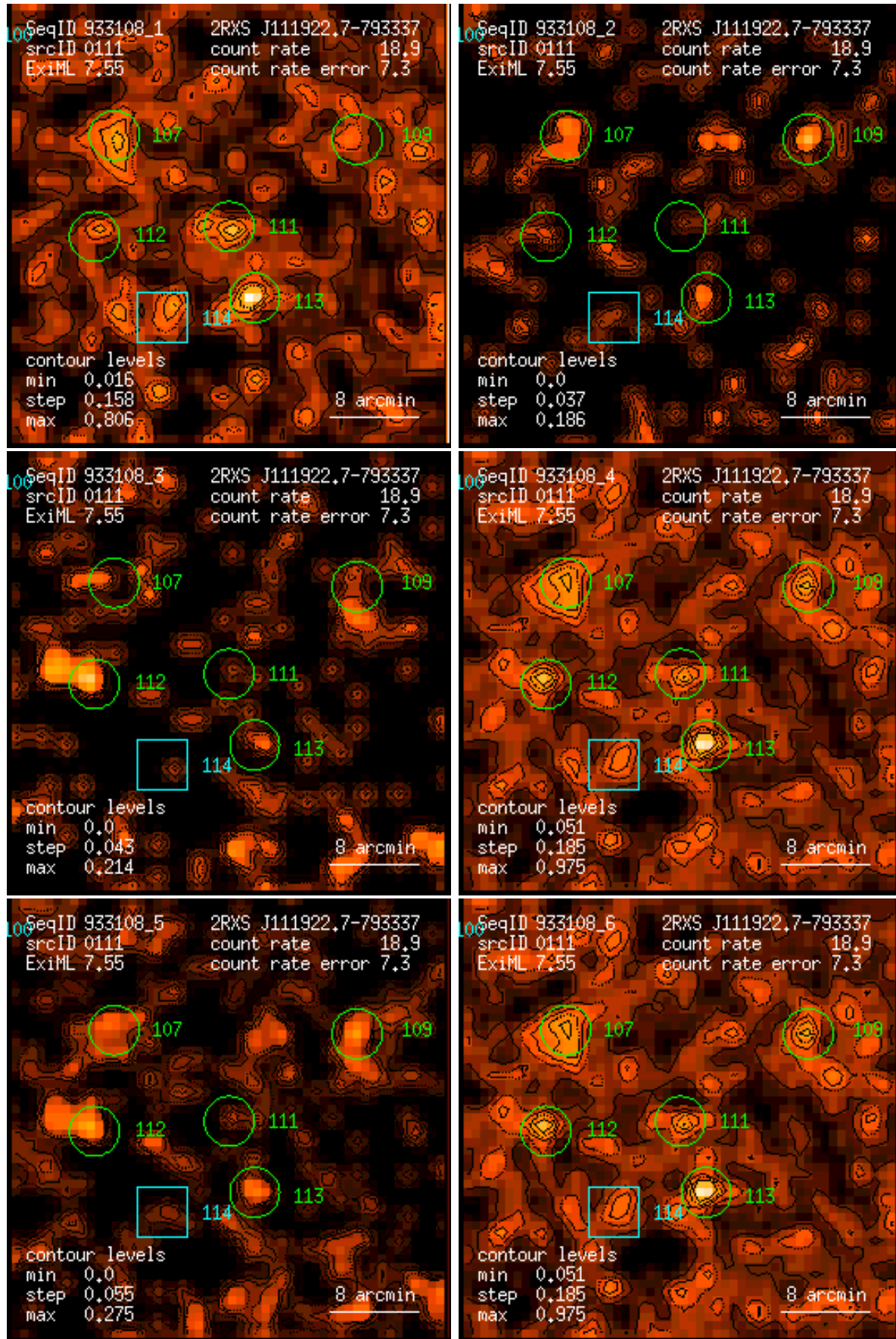
Figure 111: RASS 933108: detection 0111: band rate images, Gaussian filter: (1) PSPC channels 11 – 41, (2) 52 – 90, (3) 91 – 201, (4) 11 – 235, (5) 52 – 201, (6) 11 – 201. Broad band rates in counts/ks. Band rate contour levels in counts/ks/arcmin 2 .
