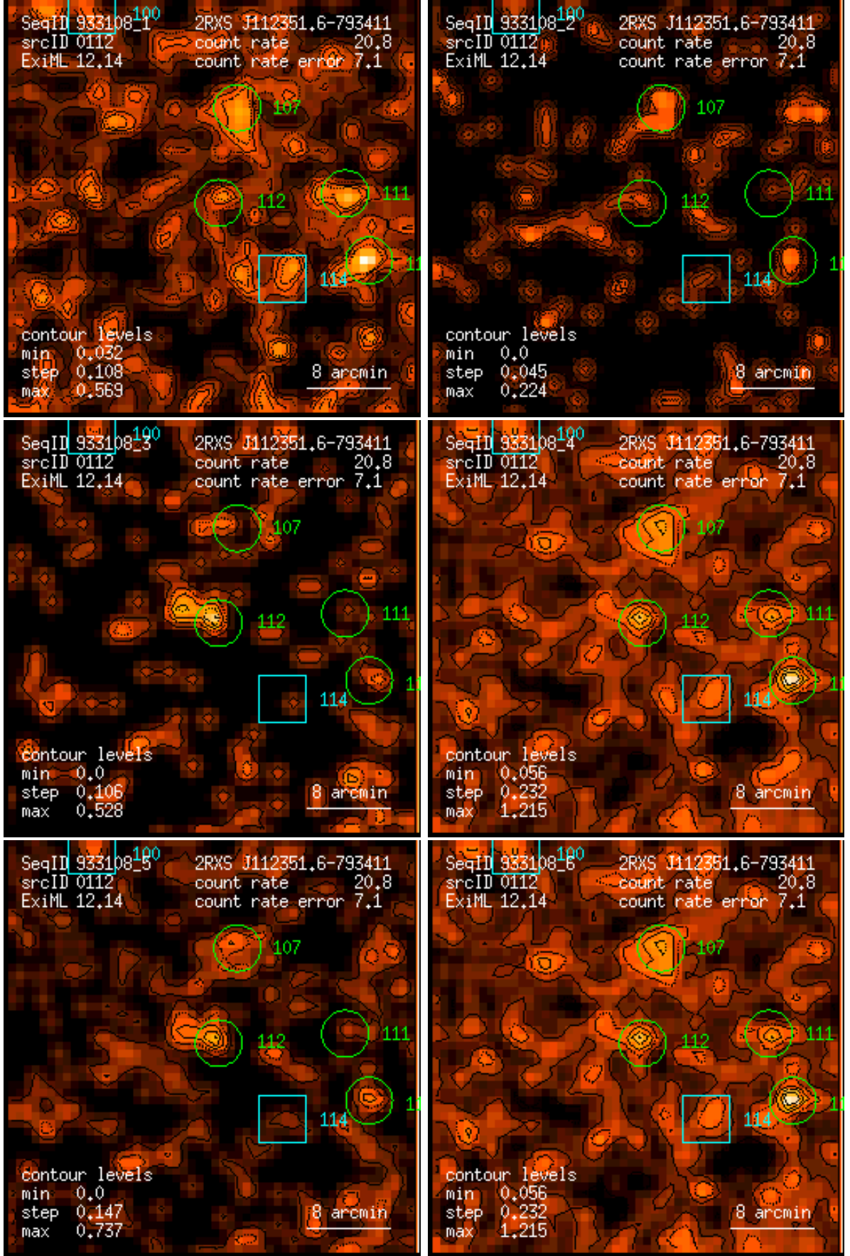
Figure 112: RASS 933108: detection 0112: band rate images, Gaussian filter: (1) PSPC channels 11 – 41, (2) 52 – 90, (3) 91 – 201, (4) 11 – 235, (5) 52 – 201, (6) 11 – 201. Broad band rates in counts/ks. Band rate contour levels in counts/ks/arcmin 2 .
