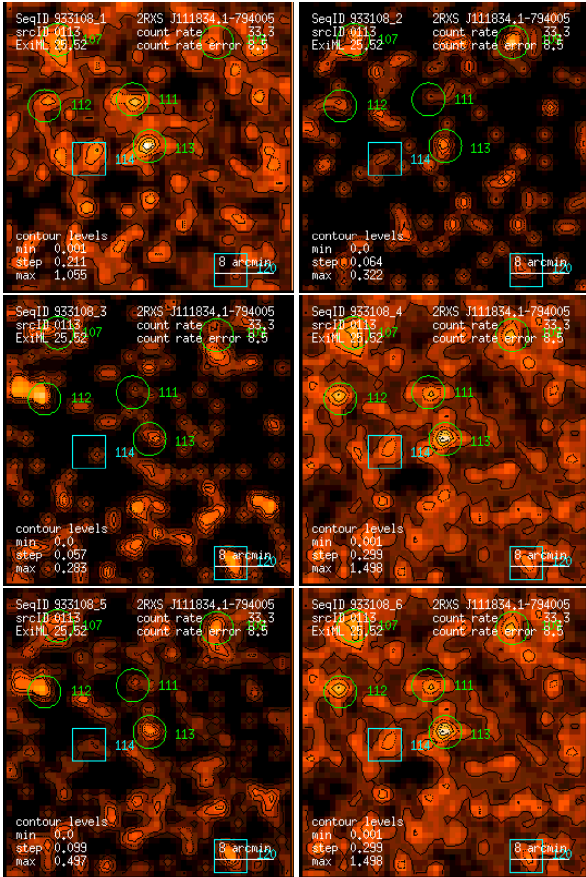
Figure 113: RASS 933108: detection 0113: band rate images, Gaussian filter: (1) PSPC channels 11 – 41, (2) 52 – 90, (3) 91 – 201, (4) 11 – 235, (5) 52 – 201, (6) 11 – 201. Broad band rates in counts/ks. Band rate contour levels in counts/ks/arcmin 2 .
