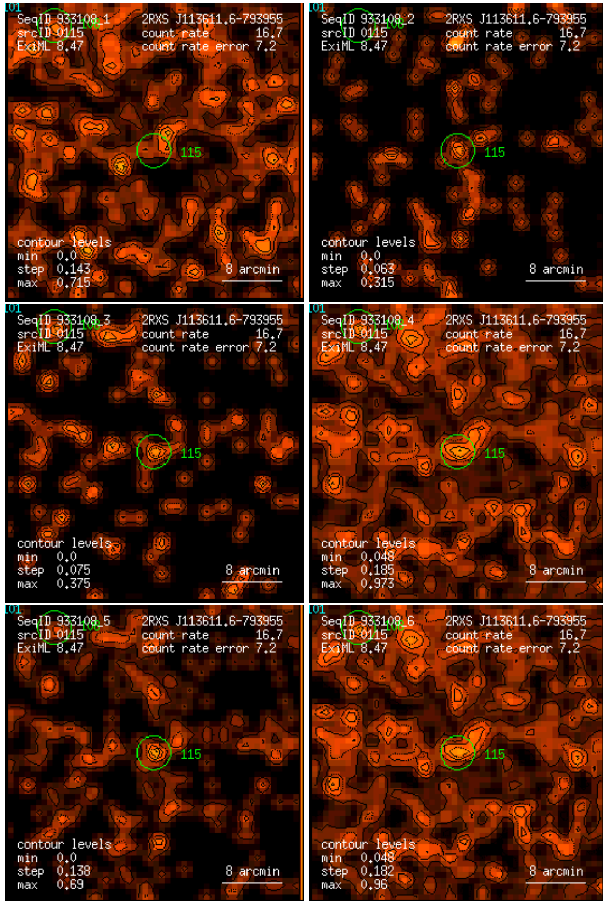
Figure 115: RASS 933108: detection 0115: band rate images, Gaussian filter: (1) PSPC channels 11 – 41, (2) 52 – 90, (3) 91 – 201, (4) 11 – 235, (5) 52 – 201, (6) 11 – 201. Broad band rates in counts/ks. Band rate contour levels in counts/ks/arcmin 2 .
