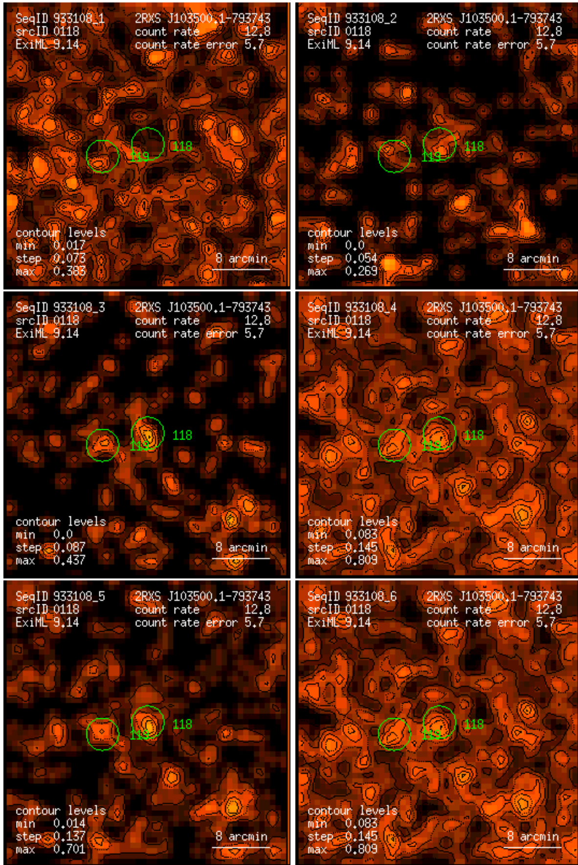
Figure 118: RASS 933108: detection 0118: band rate images, Gaussian filter: (1) PSPC channels 11 – 41, (2) 52 – 90, (3) 91 – 201, (4) 11 – 235, (5) 52 – 201, (6) 11 – 201. Broad band rates in counts/ks. Band rate contour levels in counts/ks/arcmin 2 .
