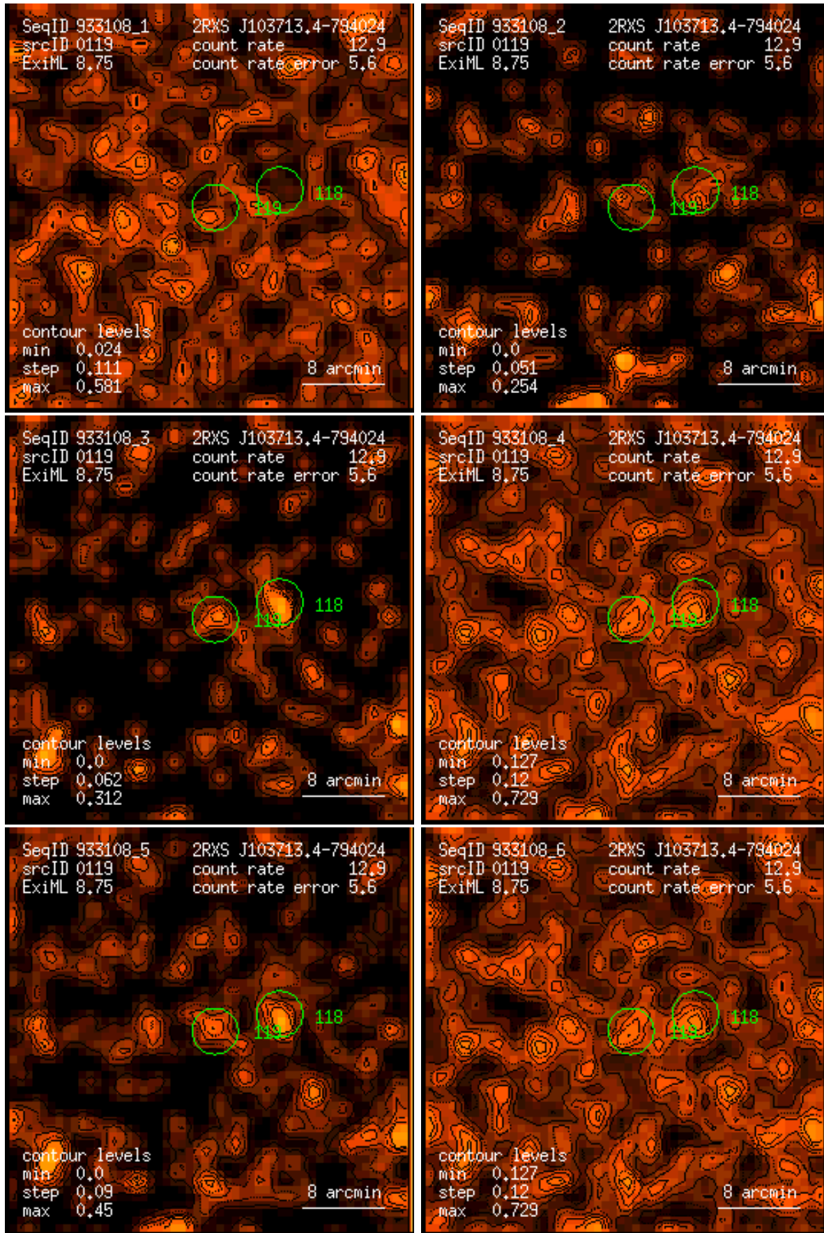
Figure 119: RASS 933108: detection 0119: band rate images, Gaussian filter: (1) PSPC channels 11 – 41, (2) 52 – 90, (3) 91 – 201, (4) 11 – 235, (5) 52 – 201, (6) 11 – 201. Broad band rates in counts/ks. Band rate contour levels in counts/ks/arcmin 2 .
