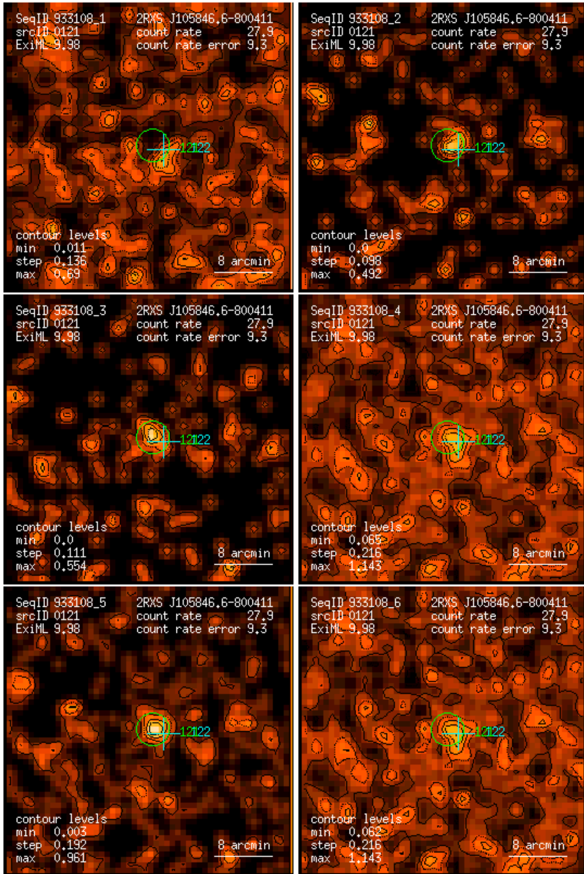
Figure 121: RASS 933108: detection 0121: band rate images, Gaussian filter: (1) PSPC channels 11 – 41, (2) 52 – 90, (3) 91 – 201, (4) 11 – 235, (5) 52 – 201, (6) 11 – 201. Broad band rates in counts/ks. Band rate contour levels in counts/ks/arcmin 2 .
