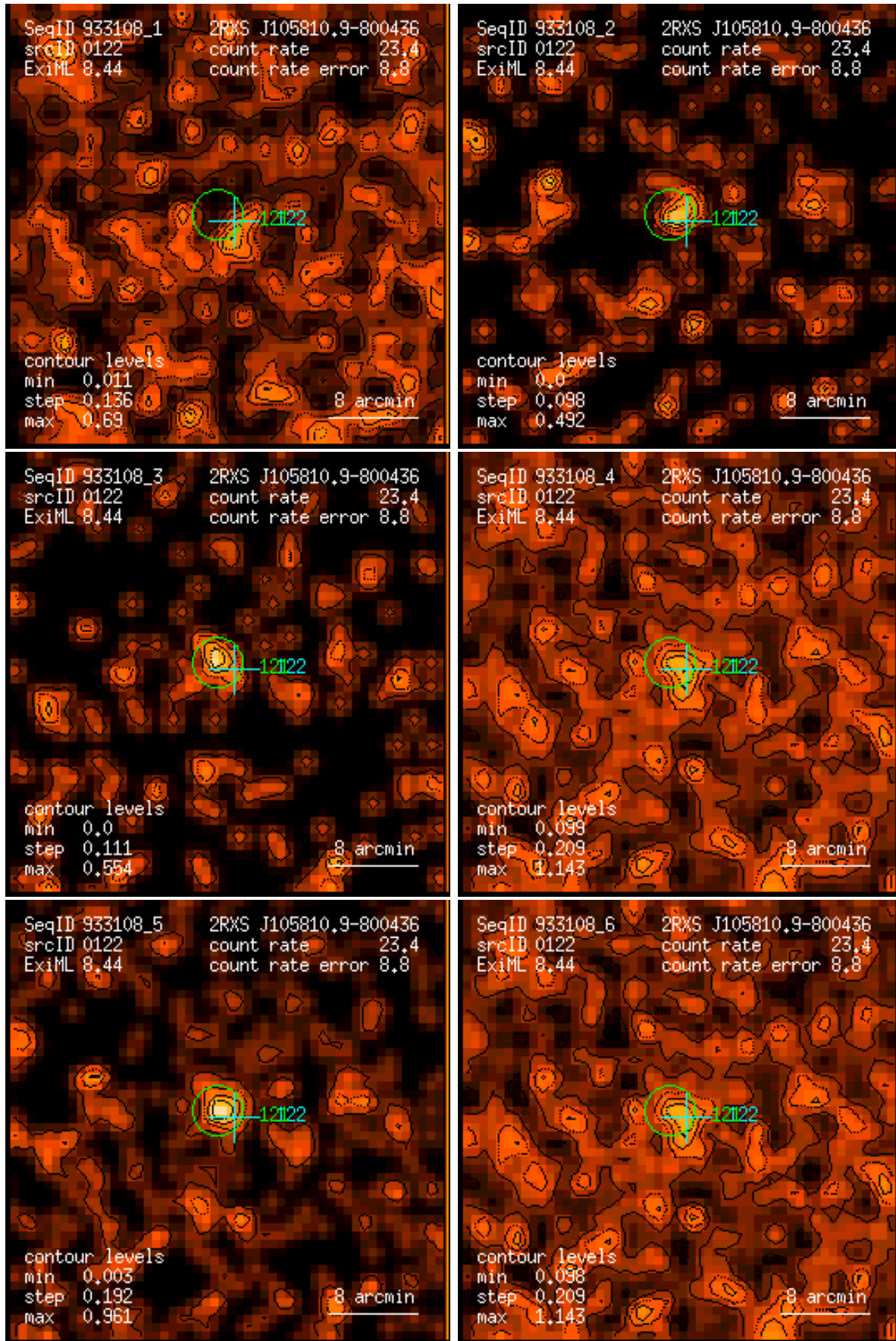
Figure 122: RASS 933108: detection 0122: band rate images, Gaussian filter: (1) PSPC channels 11 – 41, (2) 52 – 90, (3) 91 – 201, (4) 11 – 235, (5) 52 – 201, (6) 11 – 201. Broad band rates in counts/ks. Band rate contour levels in counts/ks/arcmin 2 .
