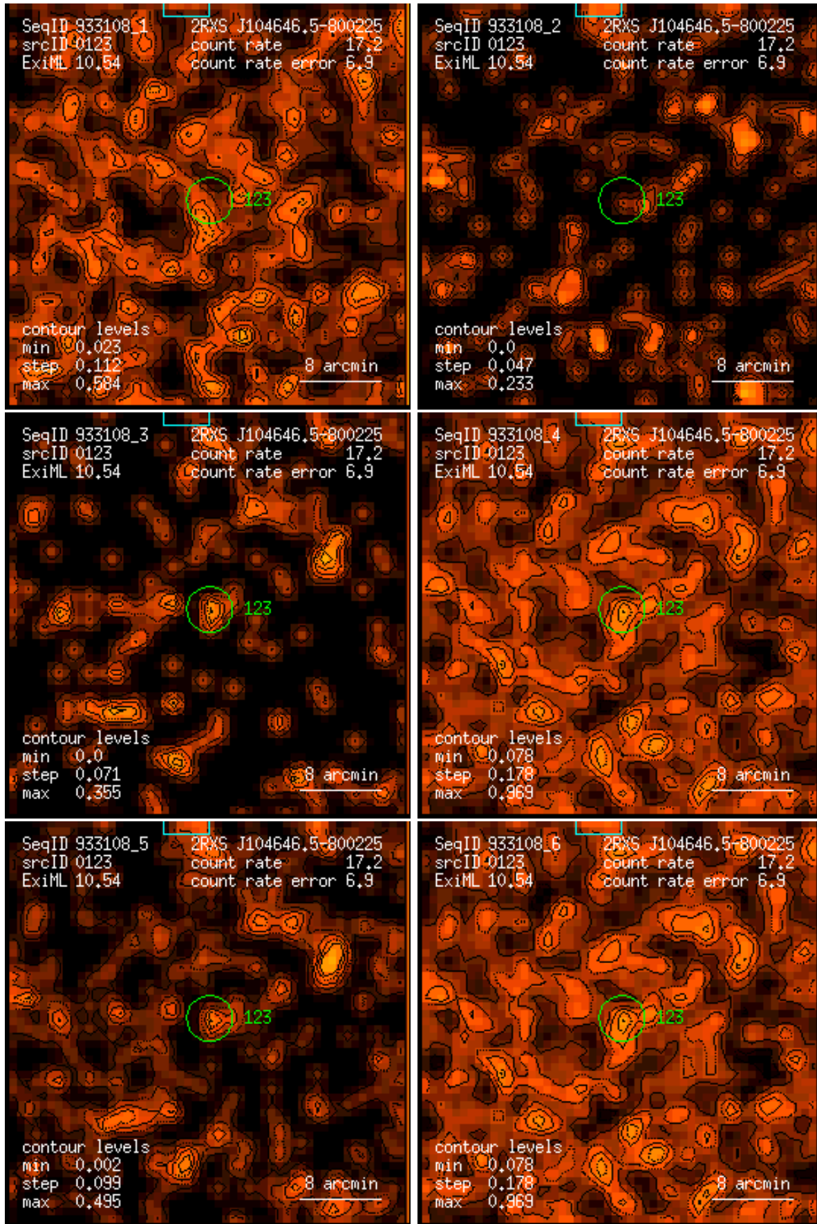
Figure 123: RASS 933108: detection 0123: band rate images, Gaussian filter: (1) PSPC channels 11 – 41, (2) 52 – 90, (3) 91 – 201, (4) 11 – 235, (5) 52 – 201, (6) 11 – 201. Broad band rates in counts/ks. Band rate contour levels in counts/ks/arcmin 2 .
