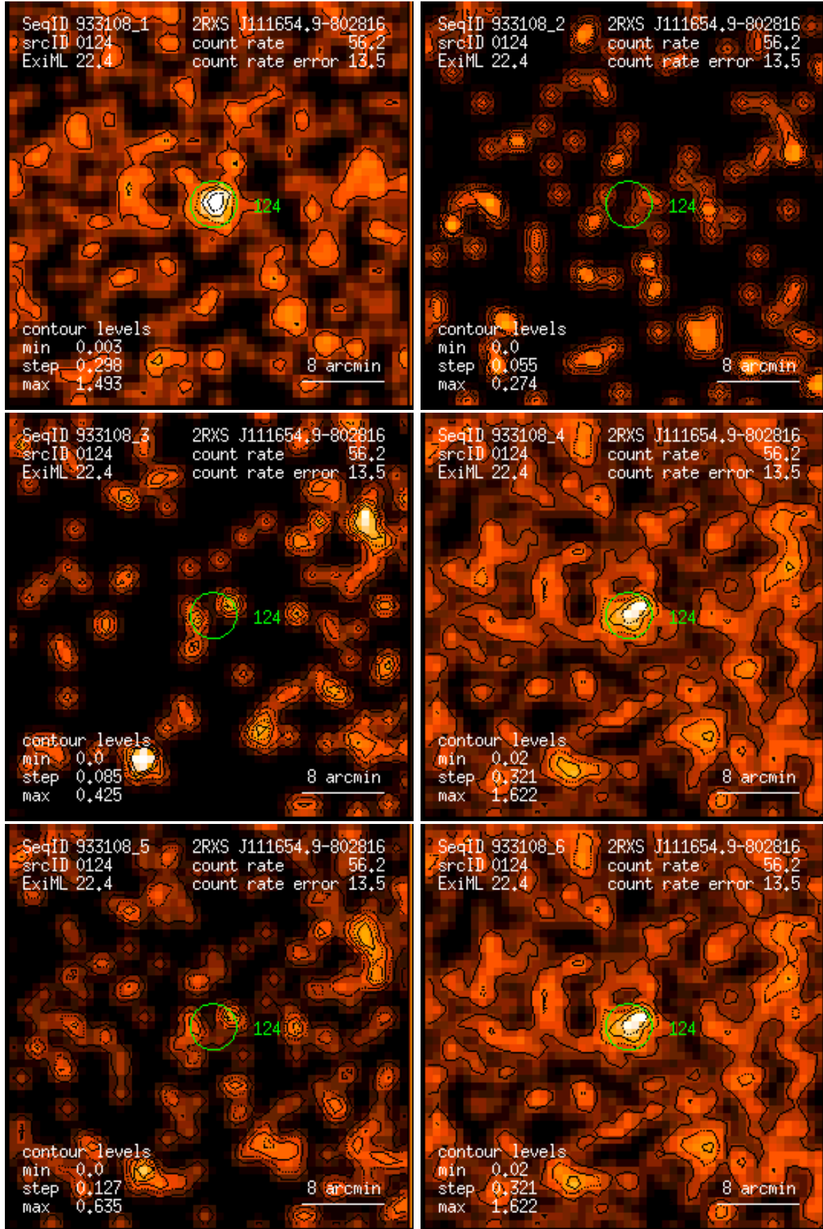
Figure 124: RASS 933108: detection 0124: band rate images, Gaussian filter: (1) PSPC channels 11 – 41, (2) 52 – 90, (3) 91 – 201, (4) 11 – 235, (5) 52 – 201, (6) 11 – 201. Broad band rates in counts/ks. Band rate contour levels in counts/ks/arcmin 2 .
