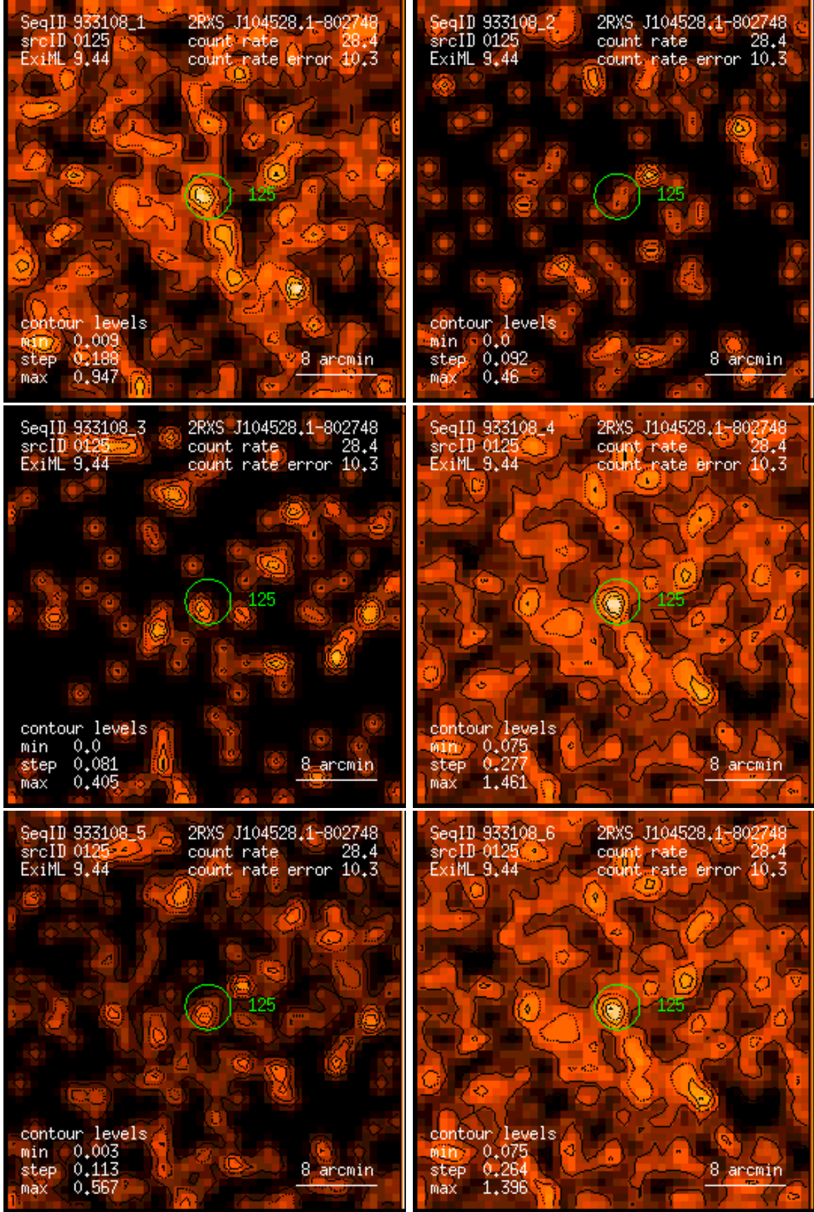
Figure 125: RASS 933108: detection 0125: band rate images, Gaussian filter: (1) PSPC channels 11 – 41, (2) 52 – 90, (3) 91 – 201, (4) 11 – 235, (5) 52 – 201, (6) 11 – 201. Broad band rates in counts/ks. Band rate contour levels in counts/ks/arcmin 2 .
