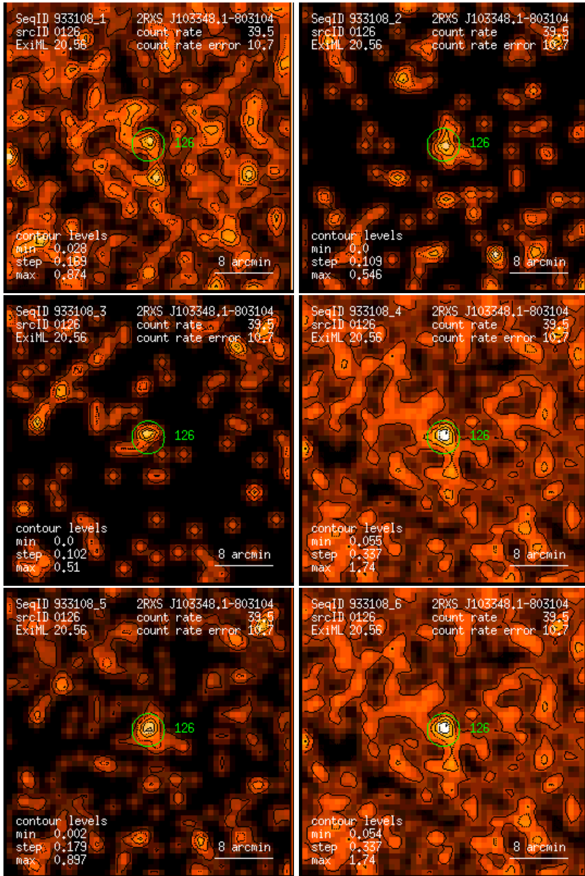
Figure 126: RASS 933108: detection 0126: band rate images, Gaussian filter: (1) PSPC channels 11 – 41, (2) 52 – 90, (3) 91 – 201, (4) 11 – 235, (5) 52 – 201, (6) 11 – 201. Broad band rates in counts/ks. Band rate contour levels in counts/ks/arcmin 2 .
