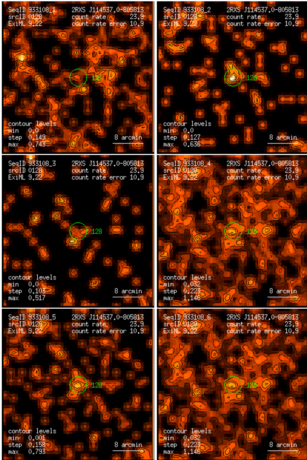
Figure 128: RASS 933108: detection 0128: band rate images, Gaussian filter: (1) PSPC channels 11 – 41, (2) 52 – 90, (3) 91 – 201, (4) 11 – 235, (5) 52 – 201, (6) 11 – 201. Broad band rates in counts/ks. Band rate contour levels in counts/ks/arcmin 2 .
