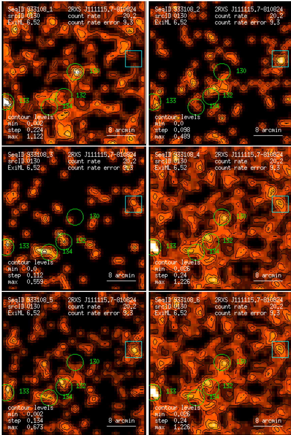
Figure 130: RASS 933108: detection 0130: band rate images, Gaussian filter: (1) PSPC channels 11 – 41, (2) 52 – 90, (3) 91 – 201, (4) 11 – 235, (5) 52 – 201, (6) 11 – 201. Broad band rates in counts/ks. Band rate contour levels in counts/ks/arcmin 2 .
