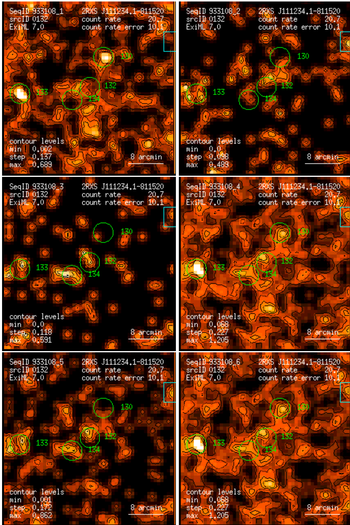
Figure 132: RASS 933108: detection 0132: band rate images, Gaussian filter: (1) PSPC channels 11 – 41, (2) 52 – 90, (3) 91 – 201, (4) 11 – 235, (5) 52 – 201, (6) 11 – 201. Broad band rates in counts/ks. Band rate contour levels in counts/ks/arcmin 2 .
