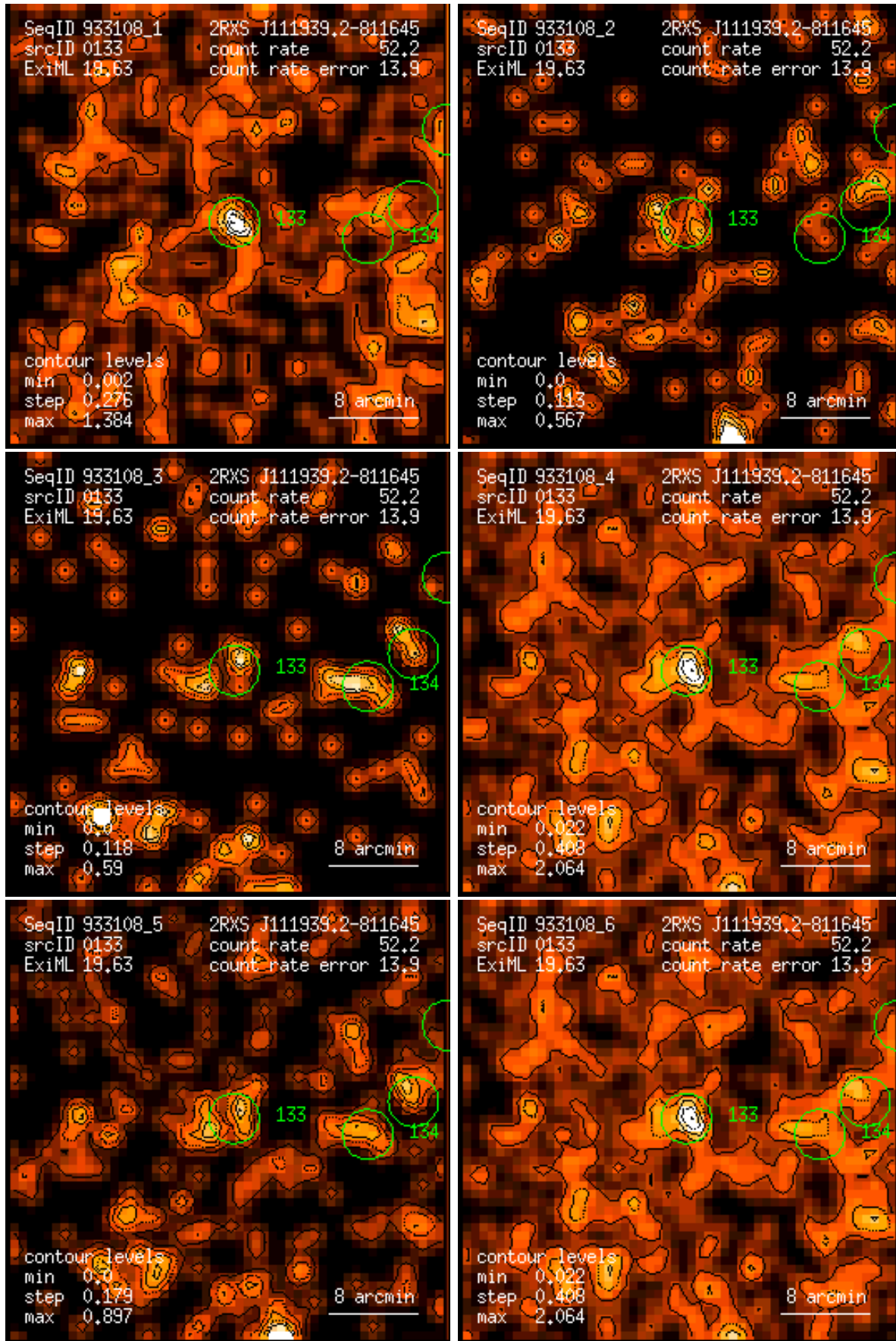
Figure 133: RASS 933108: detection 0133: band rate images, Gaussian filter: (1) PSPC channels 11 – 41, (2) 52 – 90, (3) 91 – 201, (4) 11 – 235, (5) 52 – 201, (6) 11 – 201. Broad band rates in counts/ks. Band rate contour levels in counts/ks/arcmin 2 .
