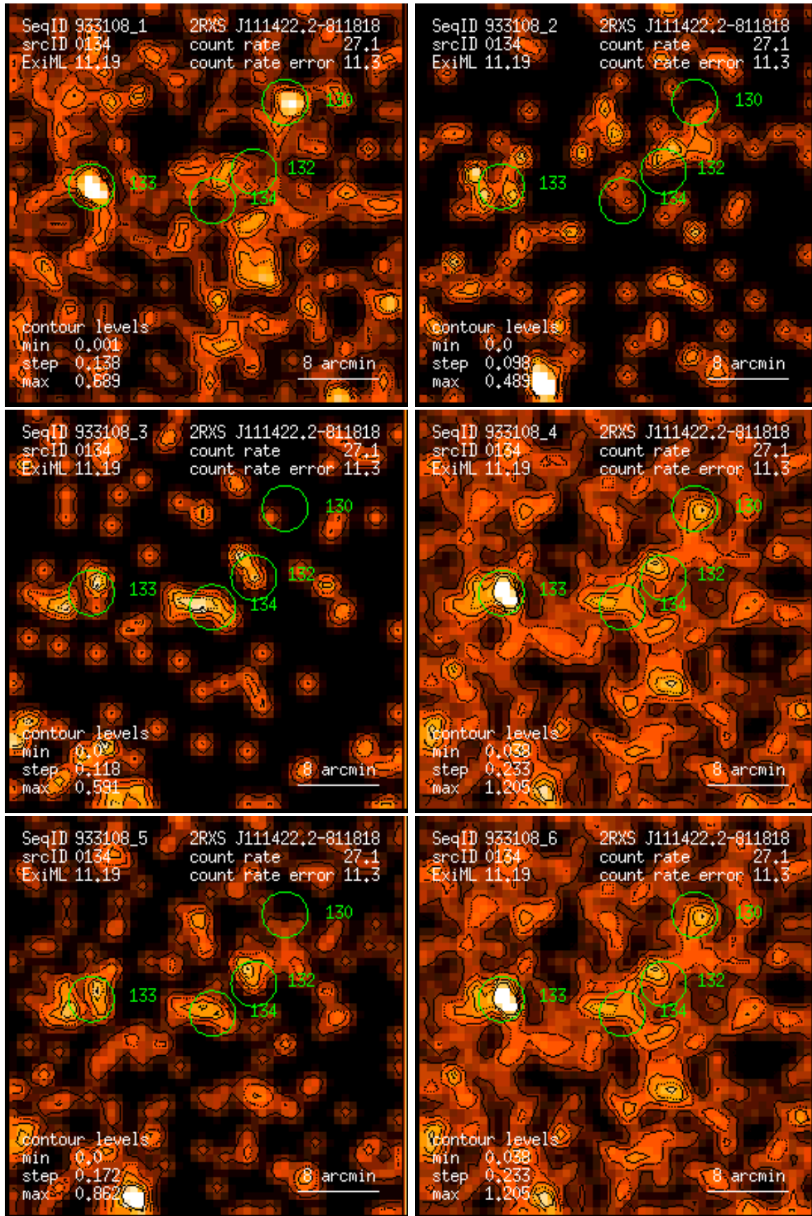
Figure 134: RASS 933108: detection 0134: band rate images, Gaussian filter: (1) PSPC channels 11 – 41, (2) 52 – 90, (3) 91 – 201, (4) 11 – 235, (5) 52 – 201, (6) 11 – 201. Broad band rates in counts/ks. Band rate contour levels in counts/ks/arcmin 2 .
