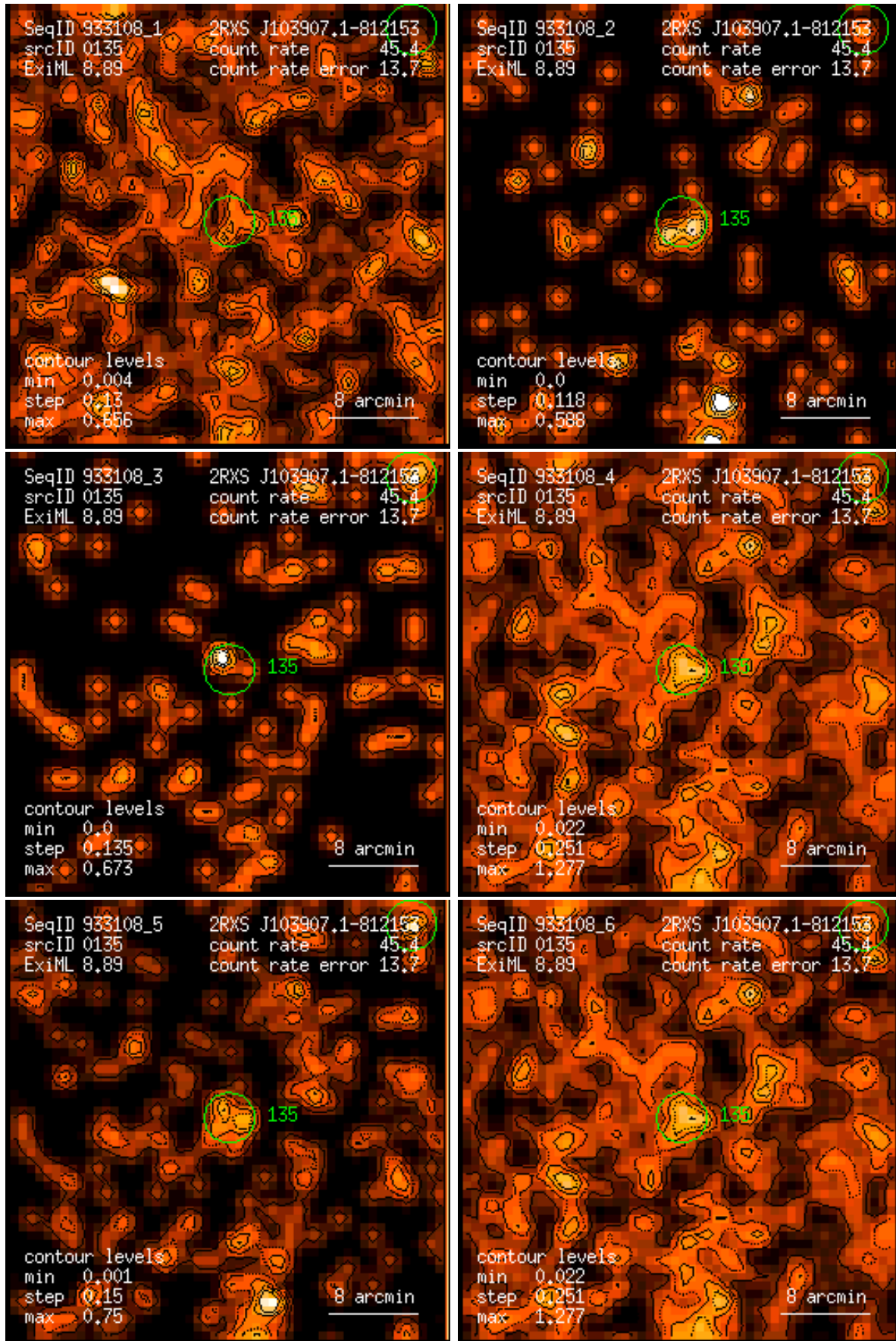
Figure 135: RASS 933108: detection 0135: band rate images, Gaussian filter: (1) PSPC channels 11 – 41, (2) 52 – 90, (3) 91 – 201, (4) 11 – 235, (5) 52 – 201, (6) 11 – 201. Broad band rates in counts/ks. Band rate contour levels in counts/ks/arcmin 2 .
