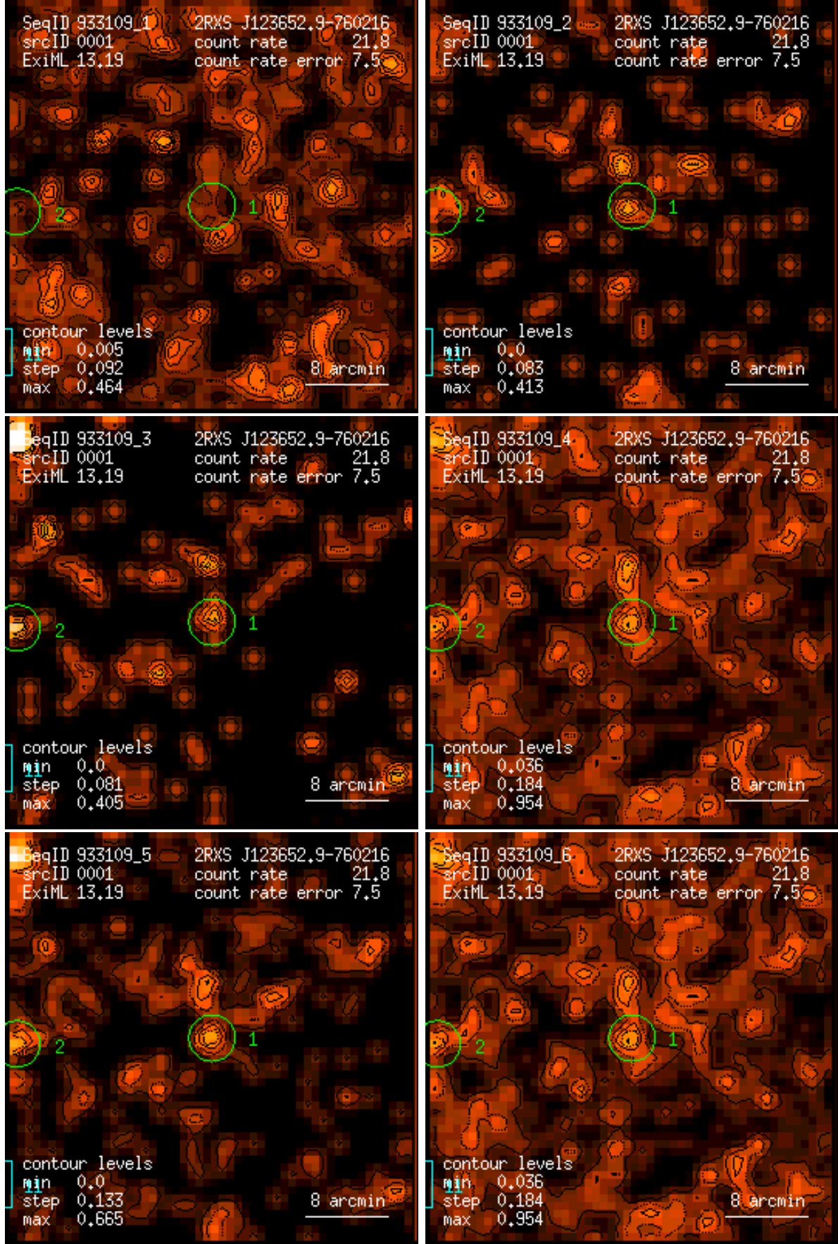
Figure 1: RASS 933109: detection 0001: band rate images, Gaussian filter: (1) PSPC channels 11 – 41, (2) 52 – 90, (3) 91 – 201, (4) 11 – 235, (5) 52 – 201, (6) 11 – 201. Broad band rates in counts/ks. Band rate contour levels in counts/ks/arcmin 2 .
