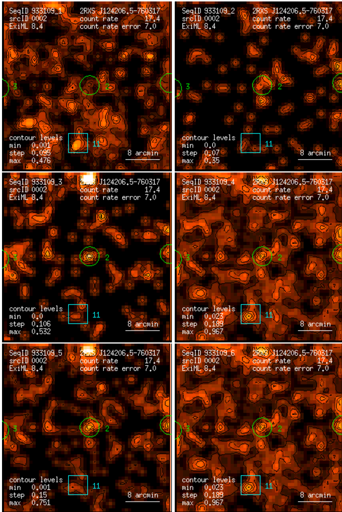
Figure 2: RASS 933109: detection 0002: band rate images, Gaussian filter: (1) PSPC channels 11 – 41, (2) 52 – 90, (3) 91 – 201, (4) 11 – 235, (5) 52 – 201, (6) 11 – 201. Broad band rates in counts/ks. Band rate contour levels in counts/ks/arcmin 2 .
