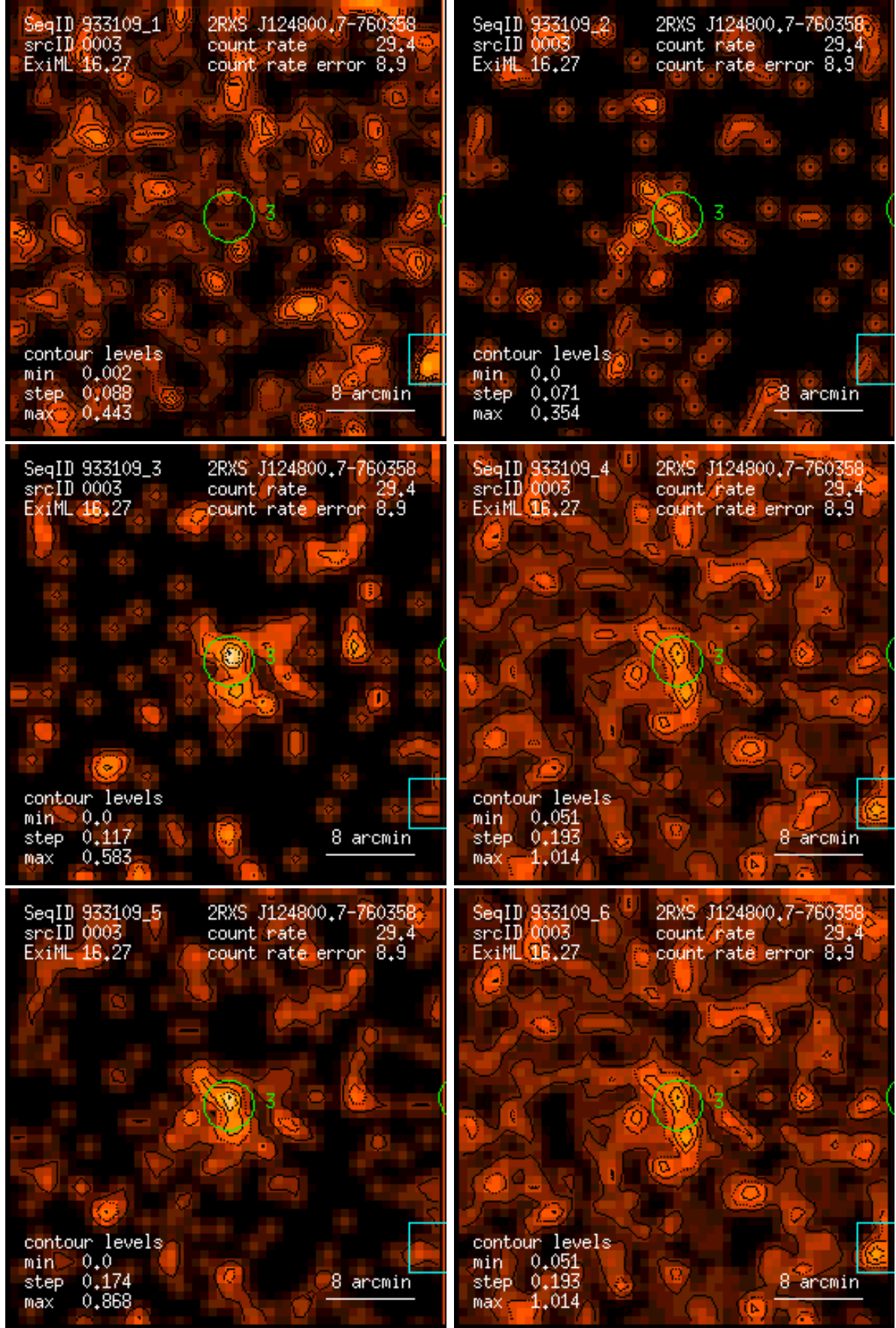
Figure 3: RASS 933109: detection 0003: band rate images, Gaussian filter: (1) PSPC channels 11 – 41, (2) 52 – 90, (3) 91 – 201, (4) 11 – 235, (5) 52 – 201, (6) 11 – 201. Broad band rates in counts/ks. Band rate contour levels in counts/ks/arcmin 2 .
