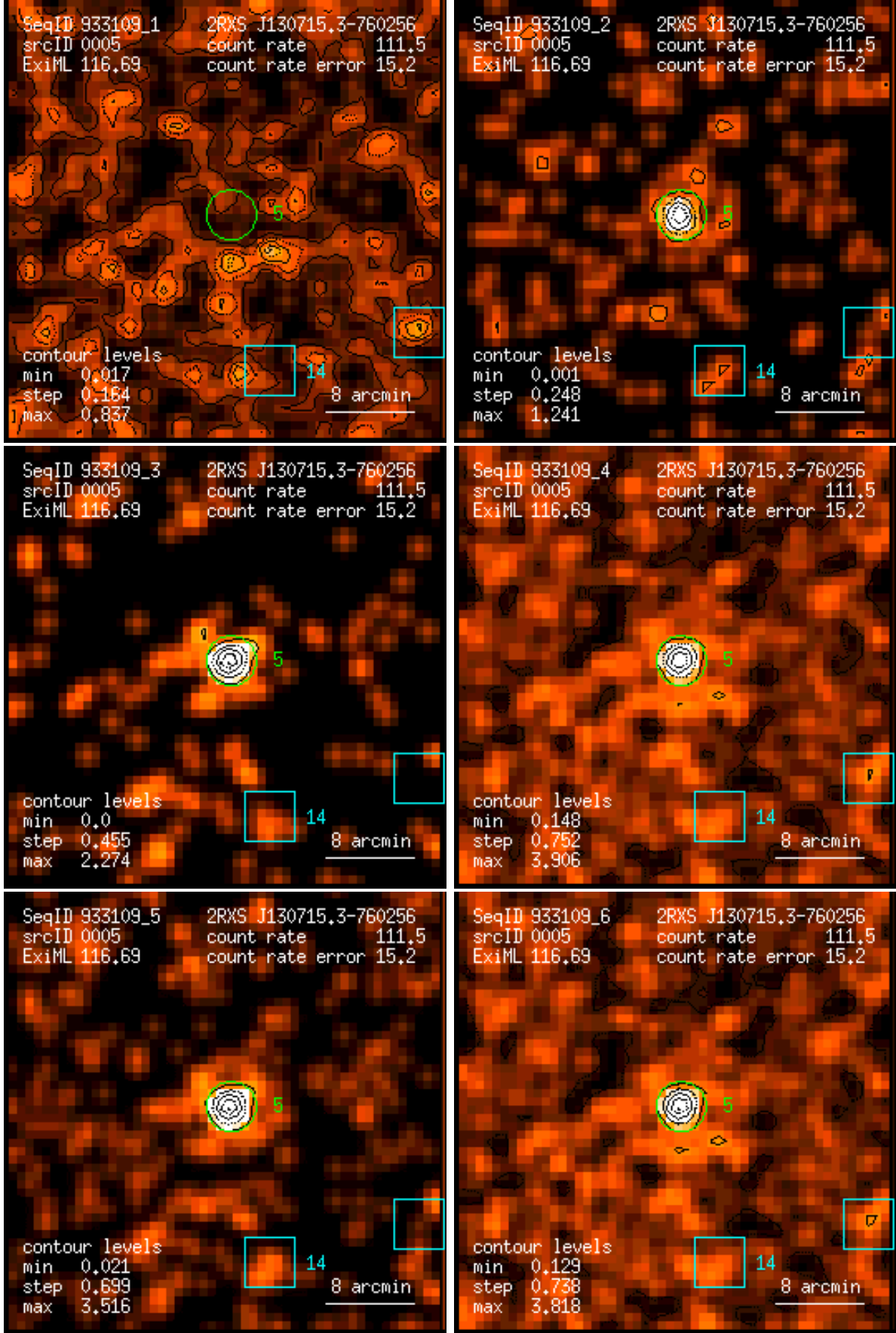
Figure 5: RASS 933109: detection 0005: band rate images, Gaussian filter: (1) PSPC channels 11 – 41, (2) 52 – 90, (3) 91 – 201, (4) 11 – 235, (5) 52 – 201, (6) 11 – 201. Broad band rates in counts/ks. Band rate contour levels in counts/ks/arcmin 2 .
