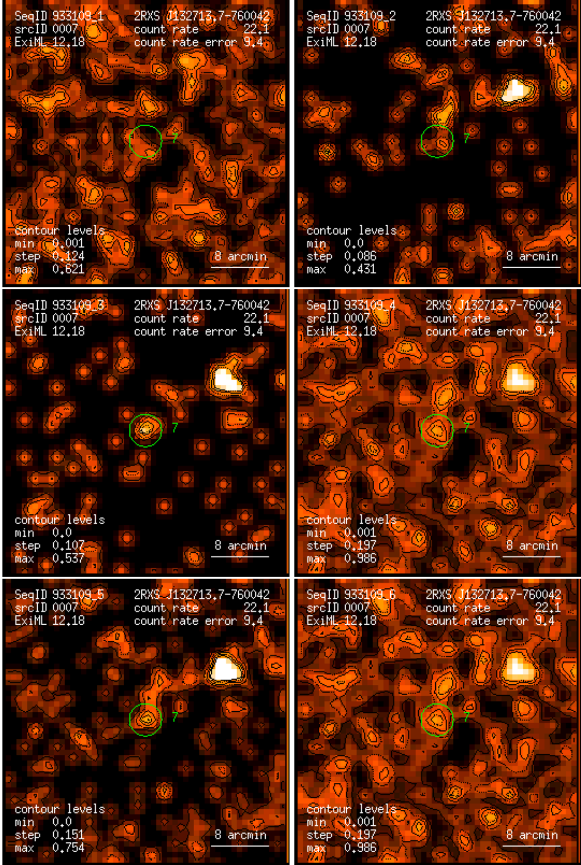
Figure 7: RASS 933109: detection 0007: band rate images, Gaussian filter: (1) PSPC channels 11 – 41, (2) 52 – 90, (3) 91 – 201, (4) 11 – 235, (5) 52 – 201, (6) 11 – 201. Broad band rates in counts/ks. Band rate contour levels in counts/ks/arcmin 2 .
