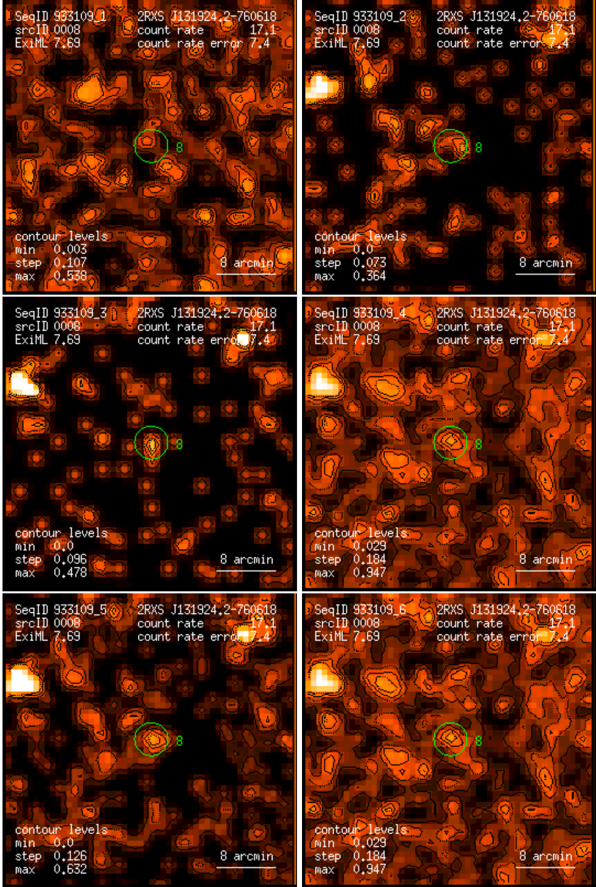
Figure 8: RASS 933109: detection 0008: band rate images, Gaussian filter: (1) PSPC channels 11 – 41, (2) 52 – 90, (3) 91 – 201, (4) 11 – 235, (5) 52 – 201, (6) 11 – 201. Broad band rates in counts/ks. Band rate contour levels in counts/ks/arcmin 2 .
