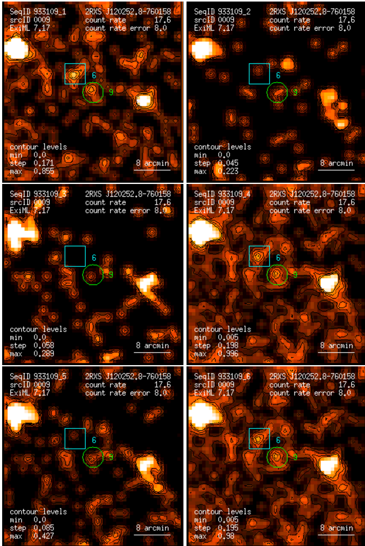
Figure 9: RASS 933109: detection 0009: band rate images, Gaussian filter: (1) PSPC channels 11 – 41, (2) 52 – 90, (3) 91 – 201, (4) 11 – 235, (5) 52 – 201, (6) 11 – 201. Broad band rates in counts/ks. Band rate contour levels in counts/ks/arcmin 2 .
