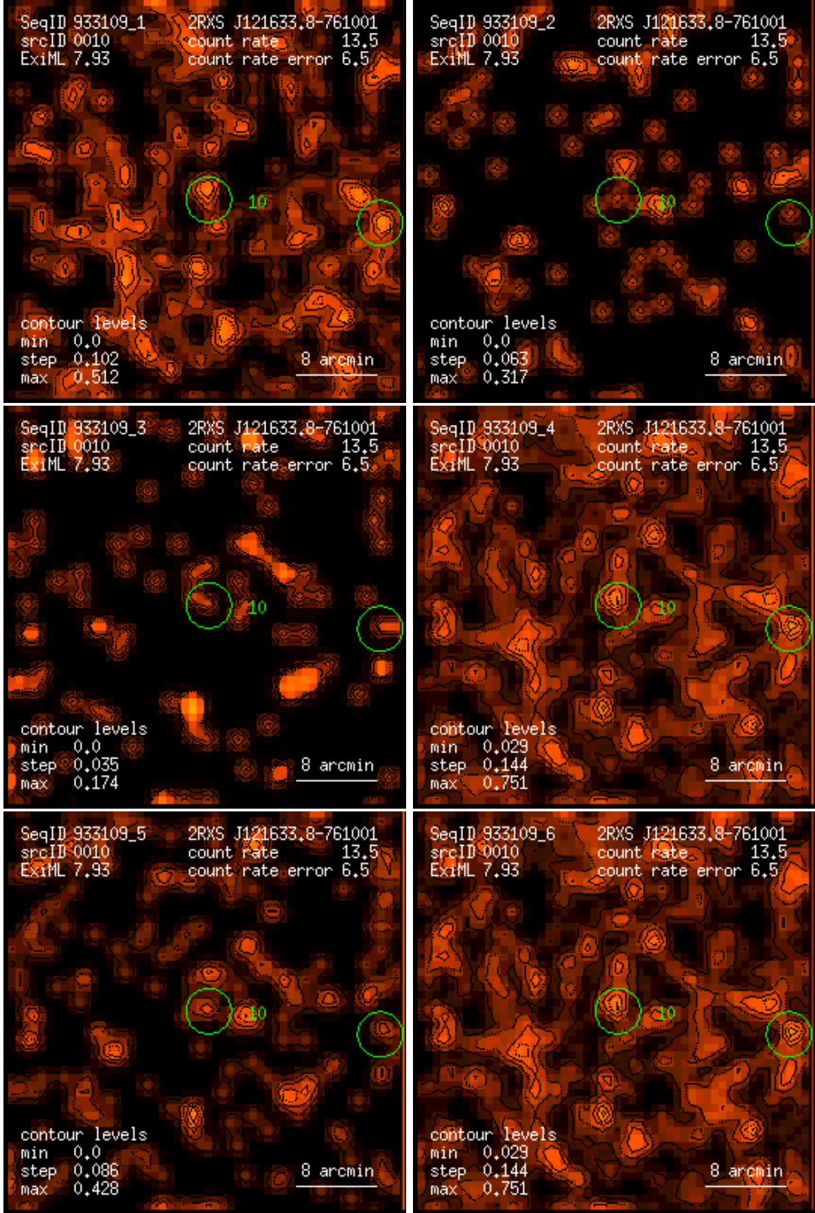
Figure 10: RASS 933109: detection 0010: band rate images, Gaussian filter: (1) PSPC channels 11 – 41, (2) 52 – 90, (3) 91 – 201, (4) 11 – 235, (5) 52 – 201, (6) 11 – 201. Broad band rates in counts/ks. Band rate contour levels in counts/ks/arcmin 2 .
