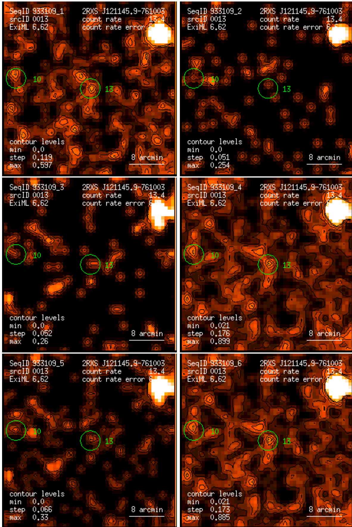
Figure 13: RASS 933109: detection 0013: band rate images, Gaussian filter: (1) PSPC channels 11 – 41, (2) 52 – 90, (3) 91 – 201, (4) 11 – 235, (5) 52 – 201, (6) 11 – 201. Broad band rates in counts/ks. Band rate contour levels in counts/ks/arcmin 2 .
