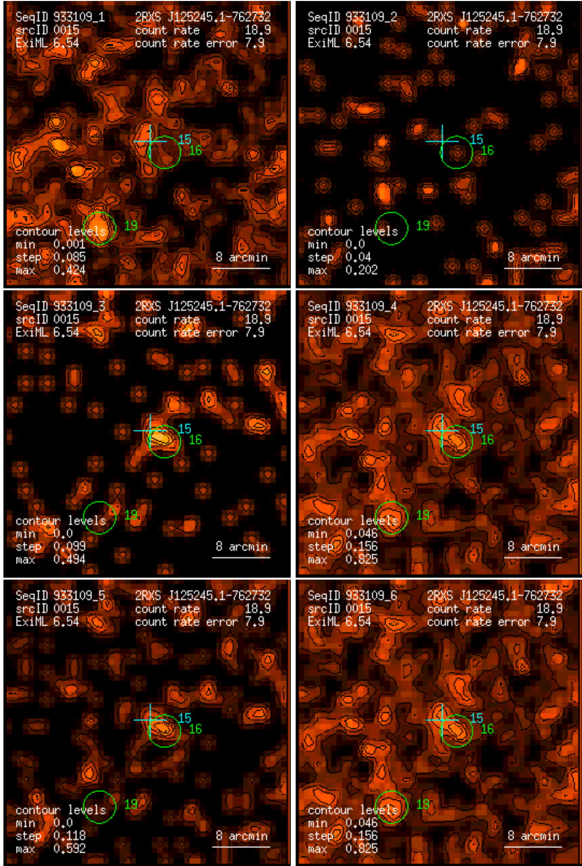
Figure 15: RASS 933109: detection 0015: band rate images, Gaussian filter: (1) PSPC channels 11 – 41, (2) 52 – 90, (3) 91 – 201, (4) 11 – 235, (5) 52 – 201, (6) 11 – 201. Broad band rates in counts/ks. Band rate contour levels in counts/ks/arcmin 2 .
