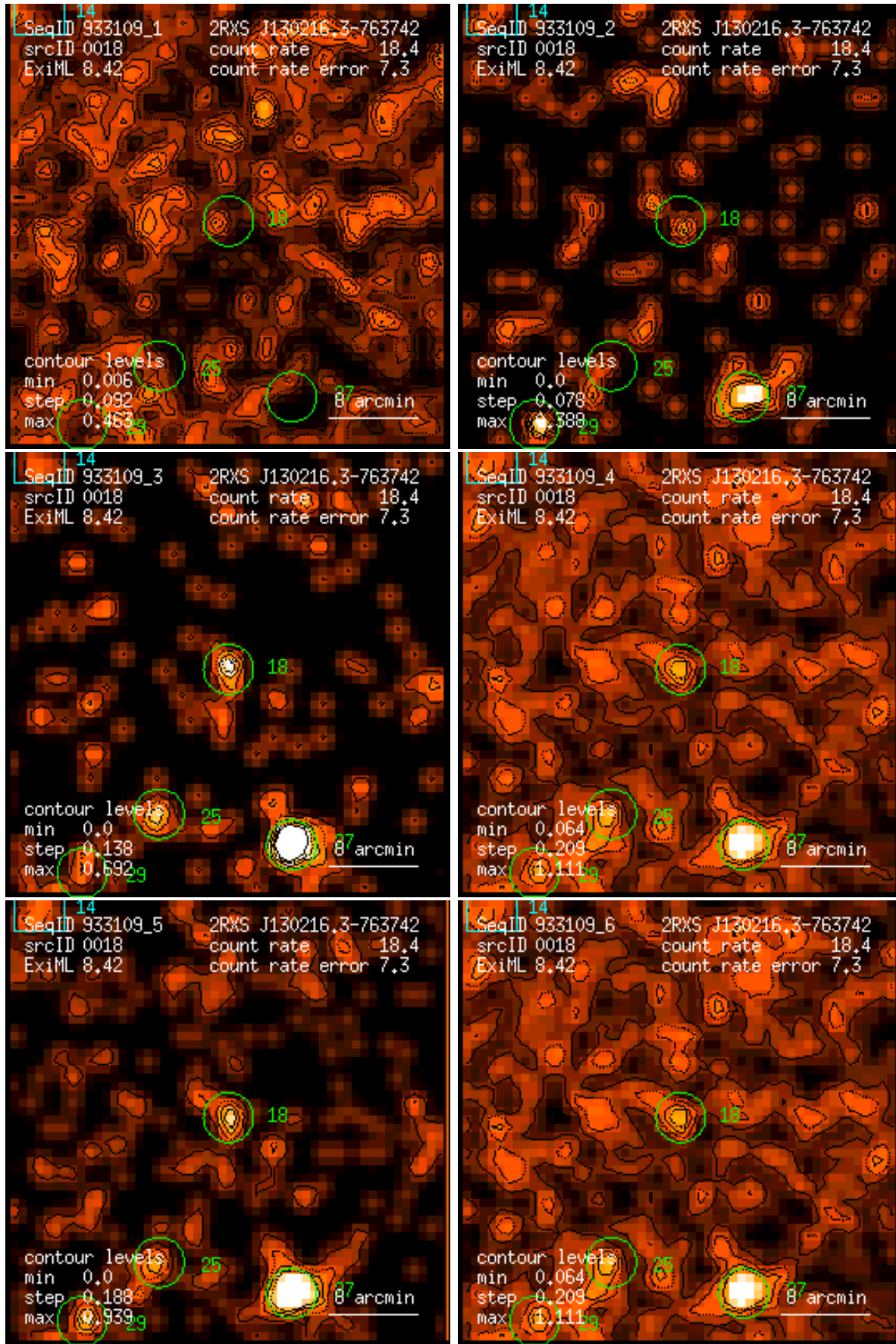
Figure 18: RASS 933109: detection 0018: band rate images, Gaussian filter: (1) PSPC channels 11 – 41, (2) 52 – 90, (3) 91 – 201, (4) 11 – 235, (5) 52 – 201, (6) 11 – 201. Broad band rates in counts/ks. Band rate contour levels in counts/ks/arcmin 2 .
