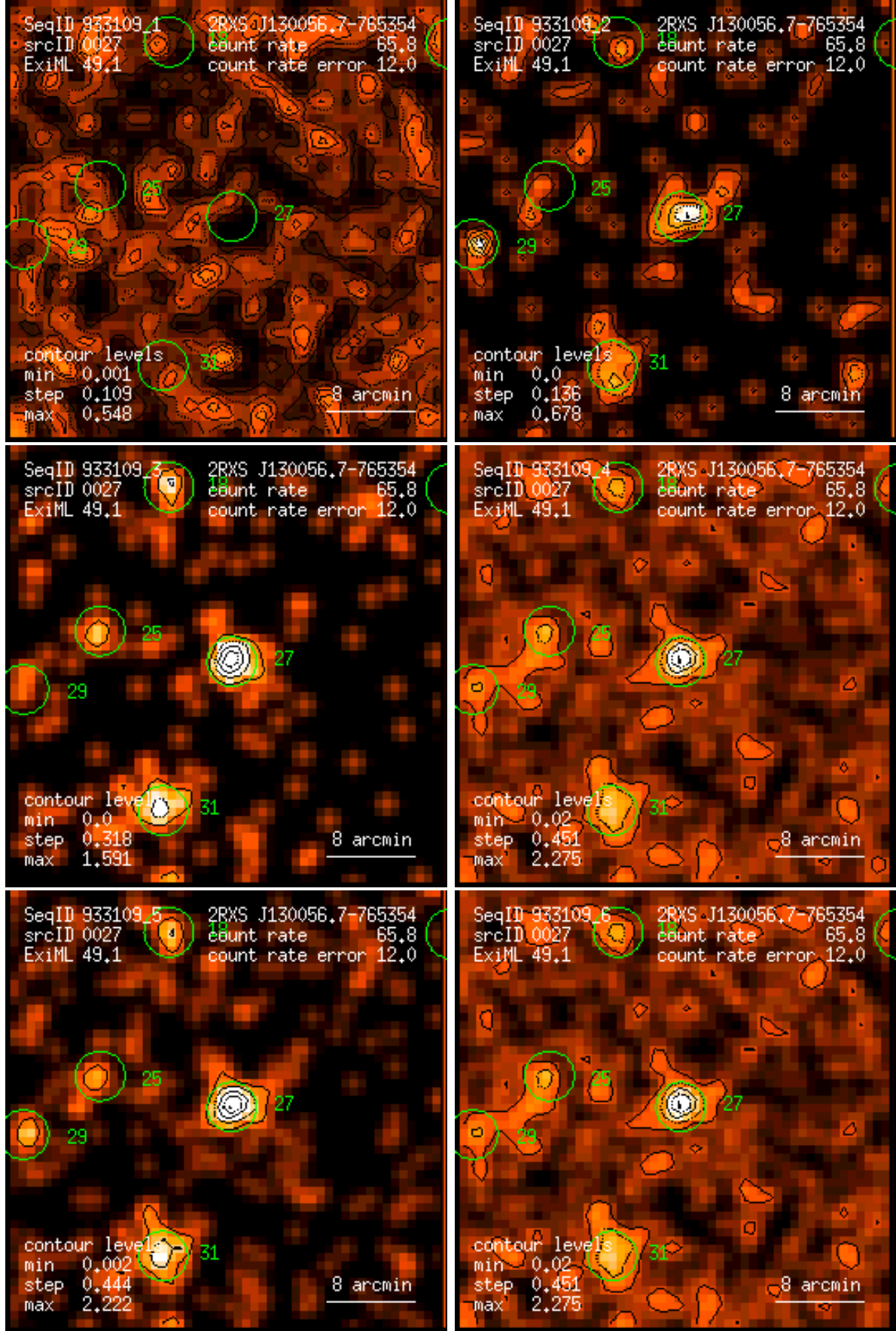
Figure 27: RASS 933109: detection 0027: band rate images, Gaussian filter: (1) PSPC channels 11 – 41, (2) 52 – 90, (3) 91 – 201, (4) 11 – 235, (5) 52 – 201, (6) 11 – 201. Broad band rates in counts/ks. Band rate contour levels in counts/ks/arcmin 2 .
