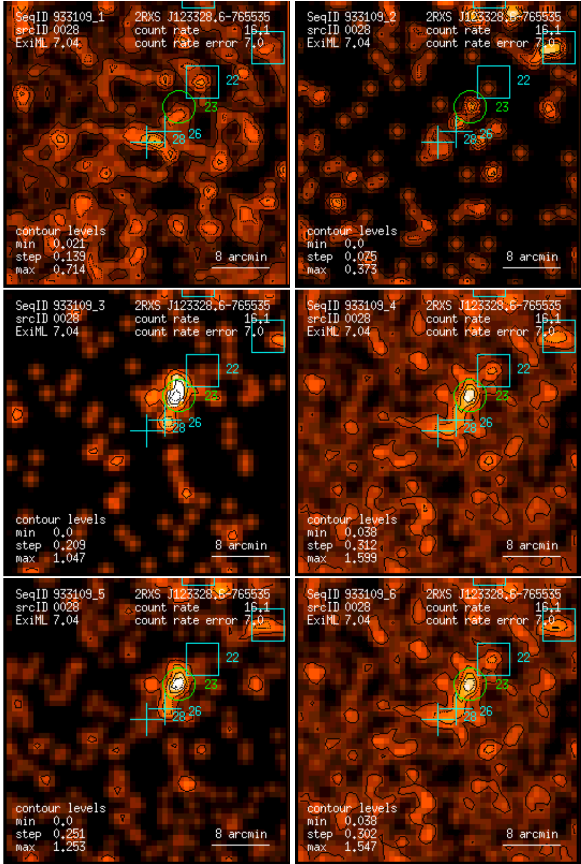
Figure 28: RASS 933109: detection 0028: band rate images, Gaussian filter: (1) PSPC channels 11 – 41, (2) 52 – 90, (3) 91 – 201, (4) 11 – 235, (5) 52 – 201, (6) 11 – 201. Broad band rates in counts/ks. Band rate contour levels in counts/ks/arcmin 2 .
