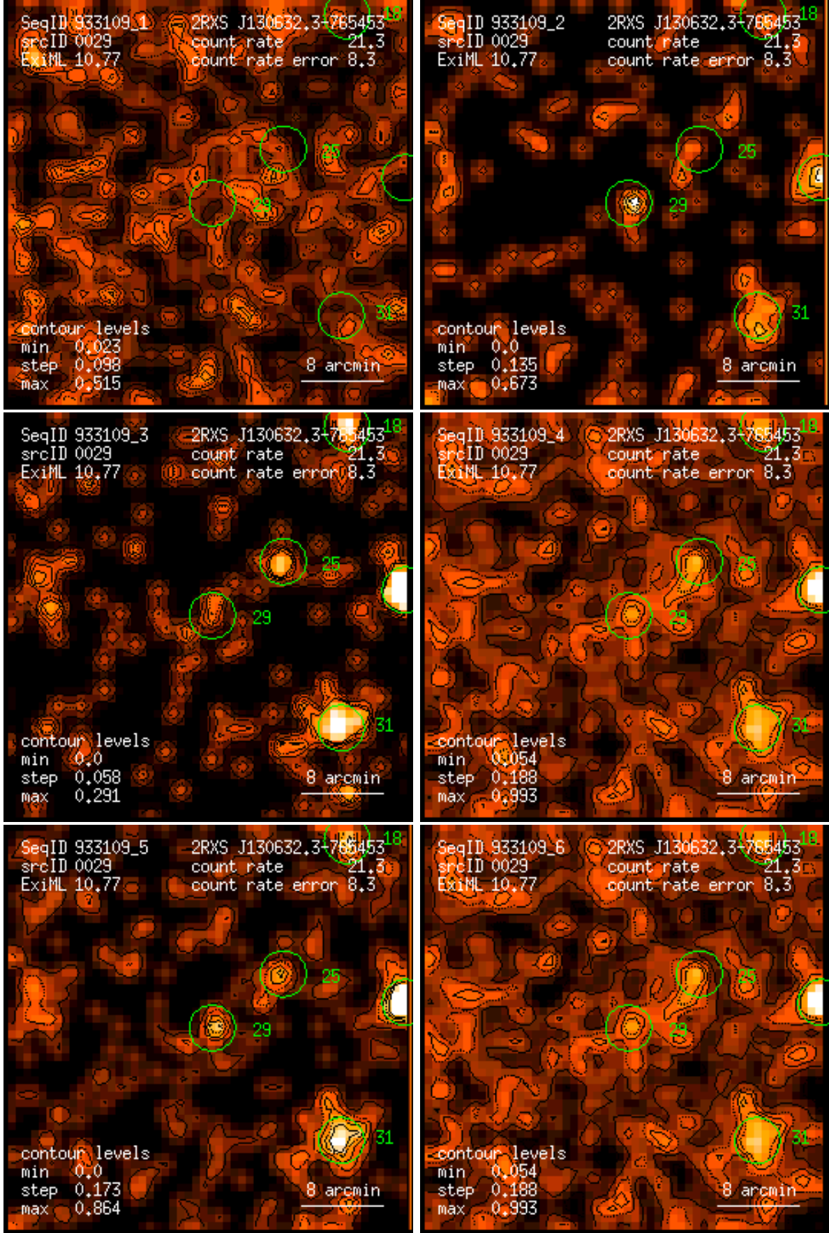
Figure 29: RASS 933109: detection 0029: band rate images, Gaussian filter: (1) PSPC channels 11 – 41, (2) 52 – 90, (3) 91 – 201, (4) 11 – 235, (5) 52 – 201, (6) 11 – 201. Broad band rates in counts/ks. Band rate contour levels in counts/ks/arcmin 2 .
