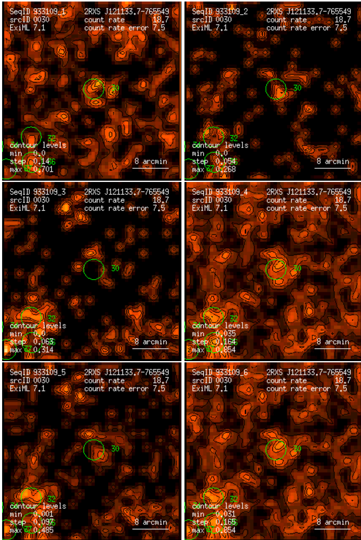
Figure 30: RASS 933109: detection 0030: band rate images, Gaussian filter: (1) PSPC channels 11 – 41, (2) 52 – 90, (3) 91 – 201, (4) 11 – 235, (5) 52 – 201, (6) 11 – 201. Broad band rates in counts/ks. Band rate contour levels in counts/ks/arcmin 2 .
