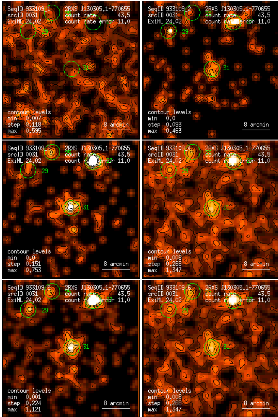
Figure 31: RASS 933109: detection 0031: band rate images, Gaussian filter: (1) PSPC channels 11 – 41, (2) 52 – 90, (3) 91 – 201, (4) 11 – 235, (5) 52 – 201, (6) 11 – 201. Broad band rates in counts/ks. Band rate contour levels in counts/ks/arcmin 2 .
