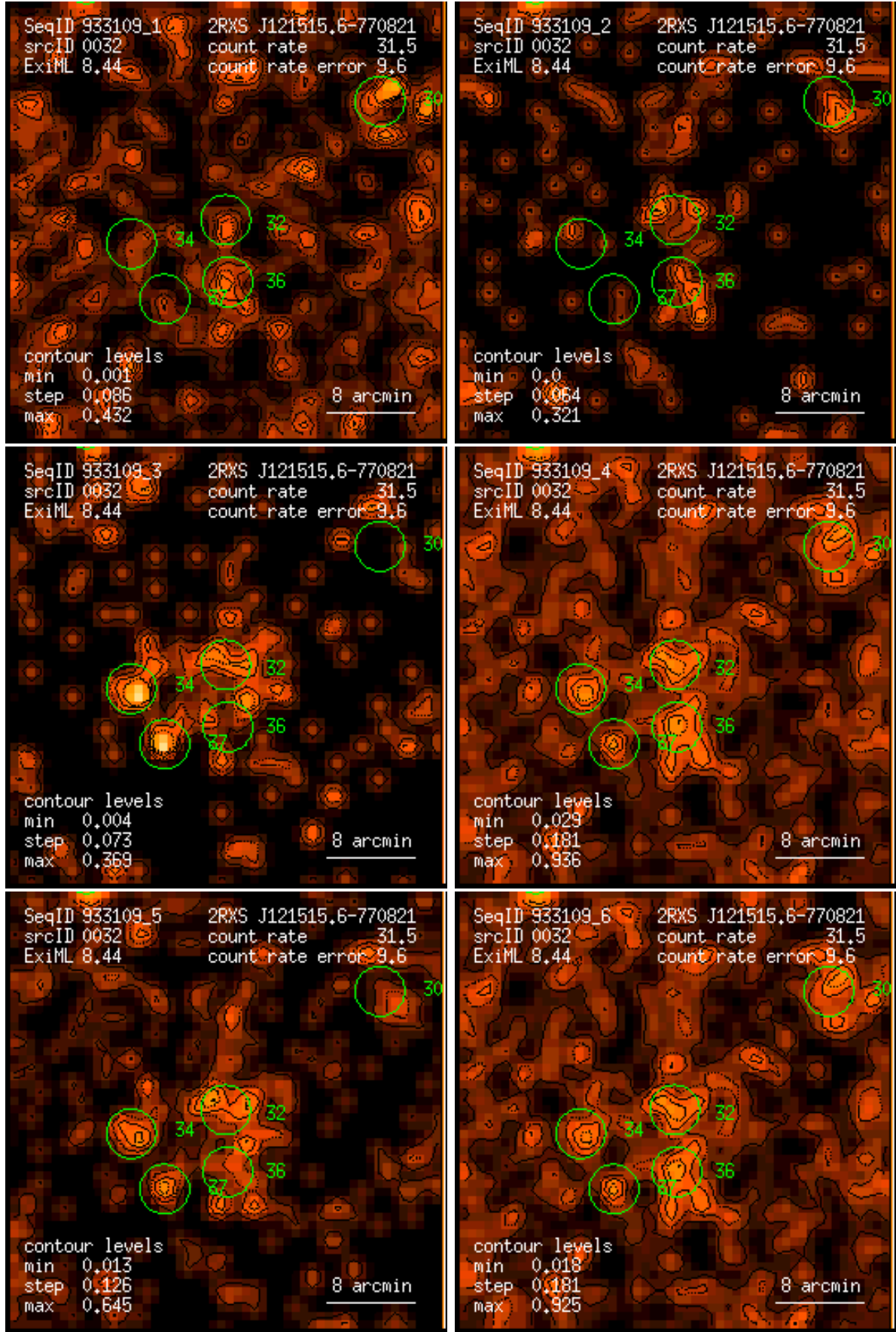
Figure 32: RASS 933109: detection 0032: band rate images, Gaussian filter: (1) PSPC channels 11 – 41, (2) 52 – 90, (3) 91 – 201, (4) 11 – 235, (5) 52 – 201, (6) 11 – 201. Broad band rates in counts/ks. Band rate contour levels in counts/ks/arcmin 2 .
