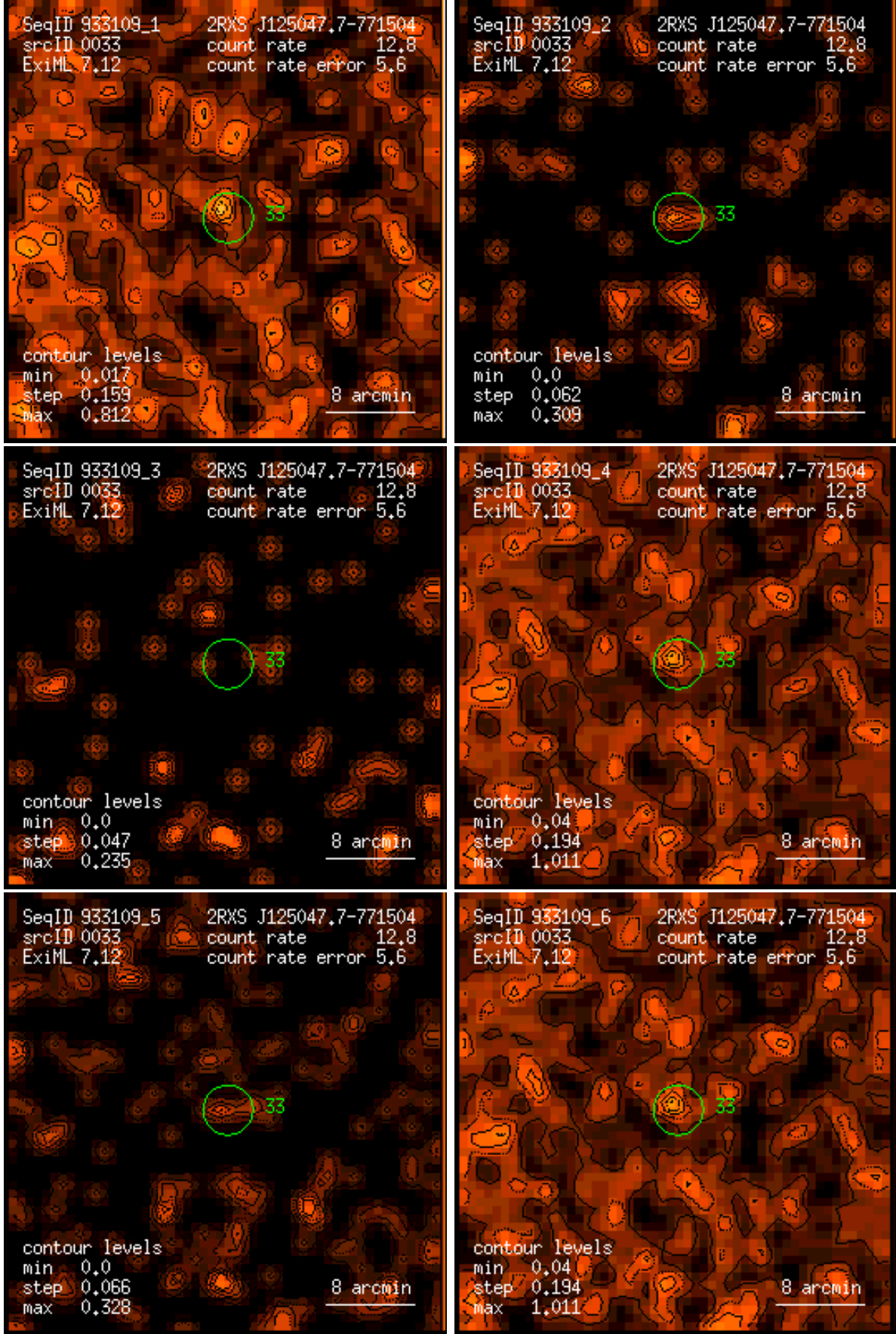
Figure 33: RASS 933109: detection 0033: band rate images, Gaussian filter: (1) PSPC channels 11 – 41, (2) 52 – 90, (3) 91 – 201, (4) 11 – 235, (5) 52 – 201, (6) 11 – 201. Broad band rates in counts/ks. Band rate contour levels in counts/ks/arcmin 2 .
