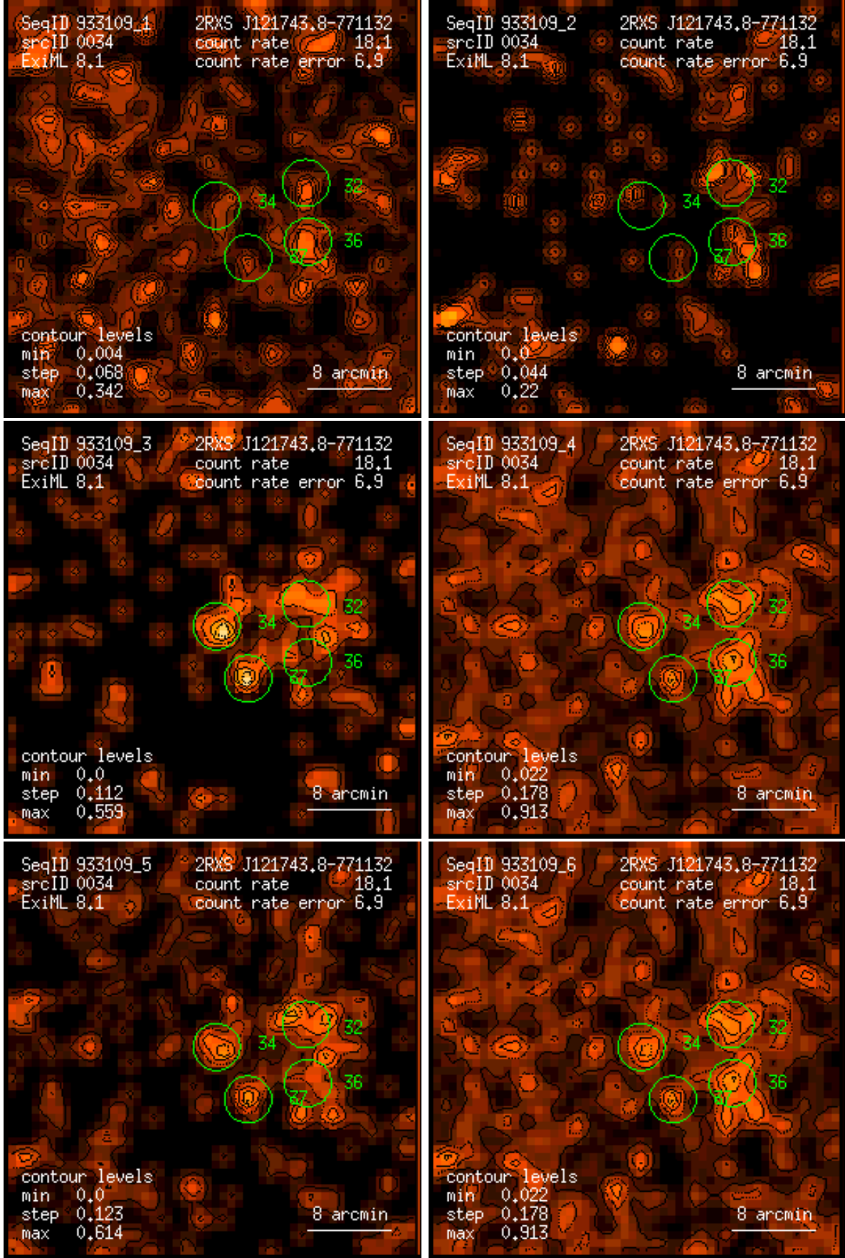
Figure 34: RASS 933109: detection 0034: band rate images, Gaussian filter: (1) PSPC channels 11 – 41, (2) 52 – 90, (3) 91 – 201, (4) 11 – 235, (5) 52 – 201, (6) 11 – 201. Broad band rates in counts/ks. Band rate contour levels in counts/ks/arcmin 2 .
