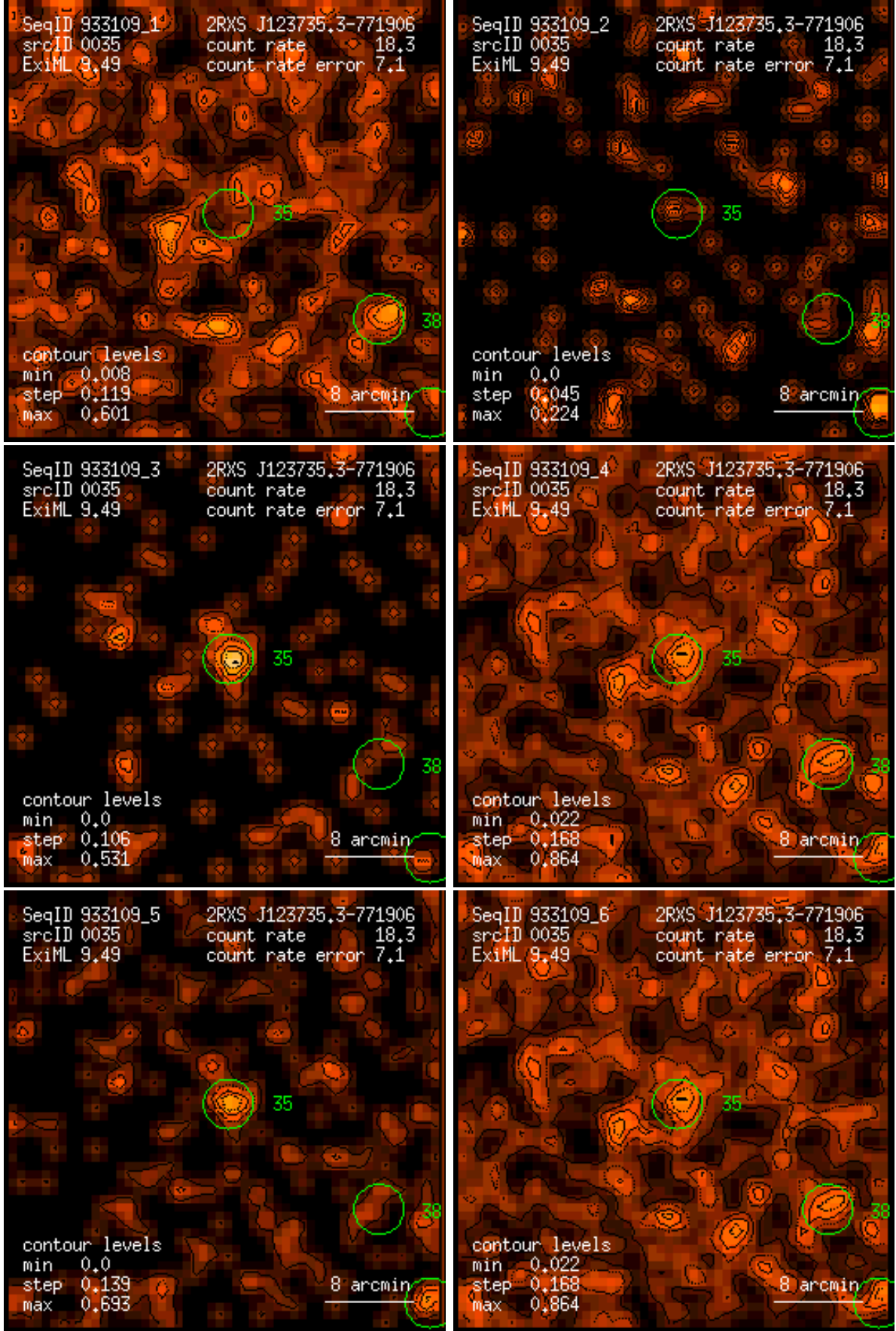
Figure 35: RASS 933109: detection 0035: band rate images, Gaussian filter: (1) PSPC channels 11 – 41, (2) 52 – 90, (3) 91 – 201, (4) 11 – 235, (5) 52 – 201, (6) 11 – 201. Broad band rates in counts/ks. Band rate contour levels in counts/ks/arcmin 2 .
