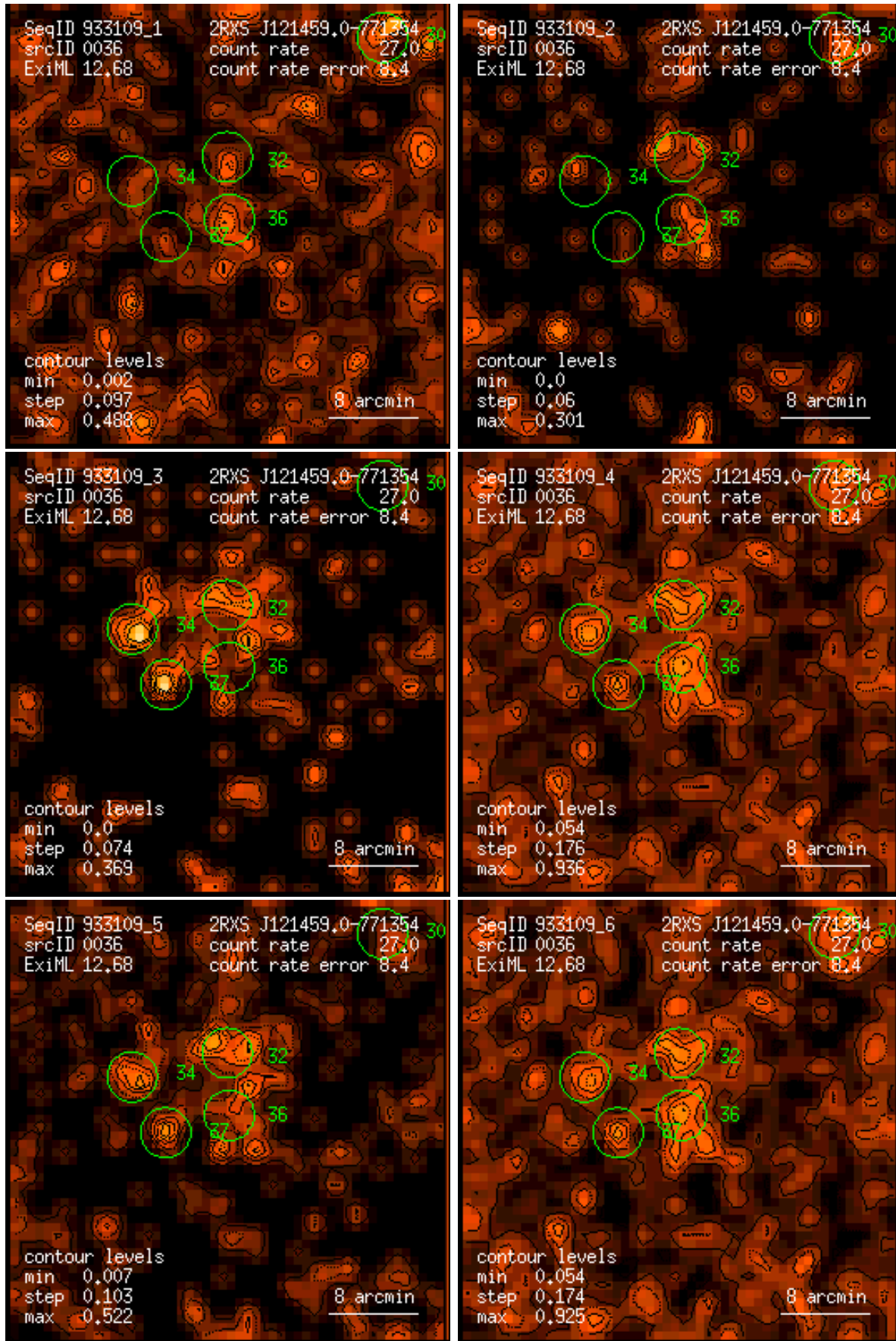
Figure 36: RASS 933109: detection 0036: band rate images, Gaussian filter: (1) PSPC channels 11 – 41, (2) 52 – 90, (3) 91 – 201, (4) 11 – 235, (5) 52 – 201, (6) 11 – 201. Broad band rates in counts/ks. Band rate contour levels in counts/ks/arcmin 2 .
