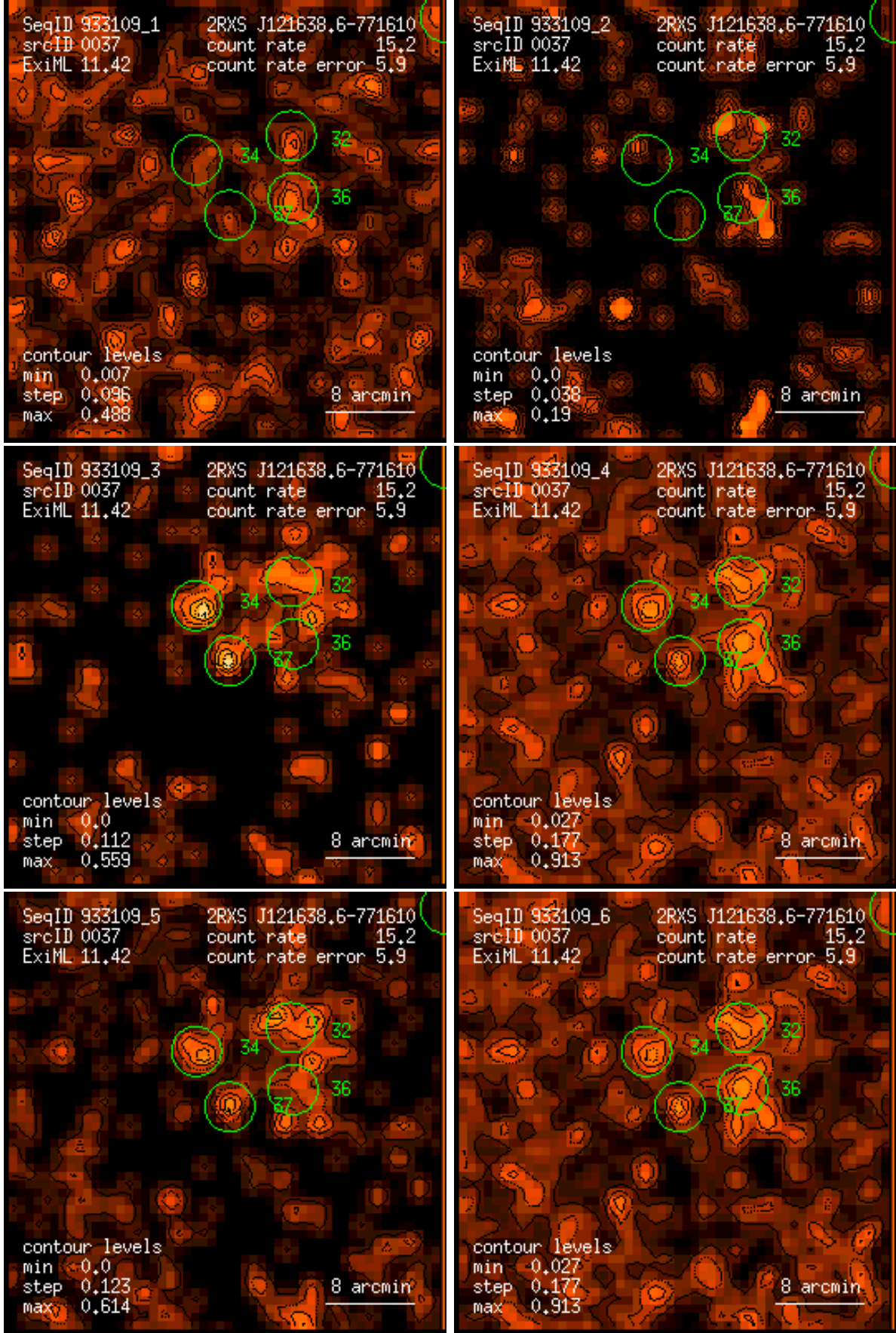
Figure 37: RASS 933109: detection 0037: band rate images, Gaussian filter: (1) PSPC channels 11 – 41, (2) 52 – 90, (3) 91 – 201, (4) 11 – 235, (5) 52 – 201, (6) 11 – 201. Broad band rates in counts/ks. Band rate contour levels in counts/ks/arcmin 2 .
