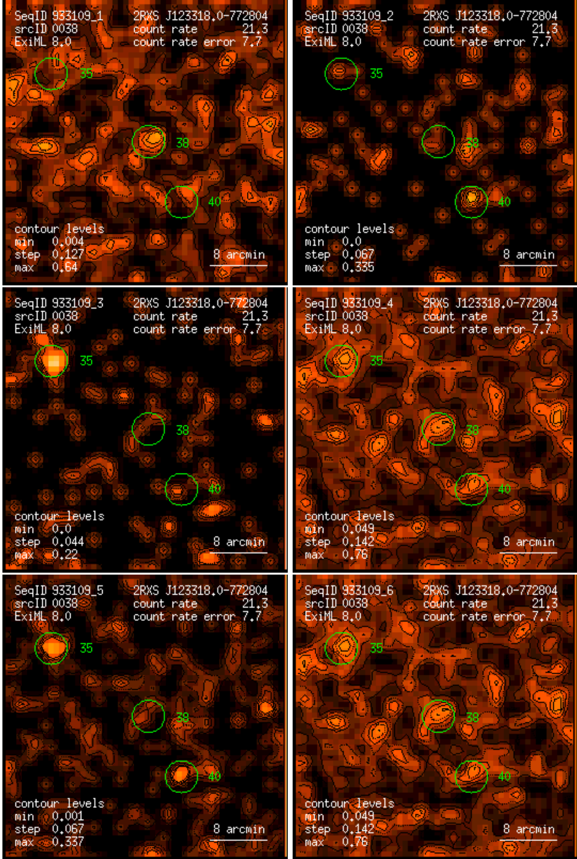
Figure 38: RASS 933109: detection 0038: band rate images, Gaussian filter: (1) PSPC channels 11 – 41, (2) 52 – 90, (3) 91 – 201, (4) 11 – 235, (5) 52 – 201, (6) 11 – 201. Broad band rates in counts/ks. Band rate contour levels in counts/ks/arcmin 2 .
