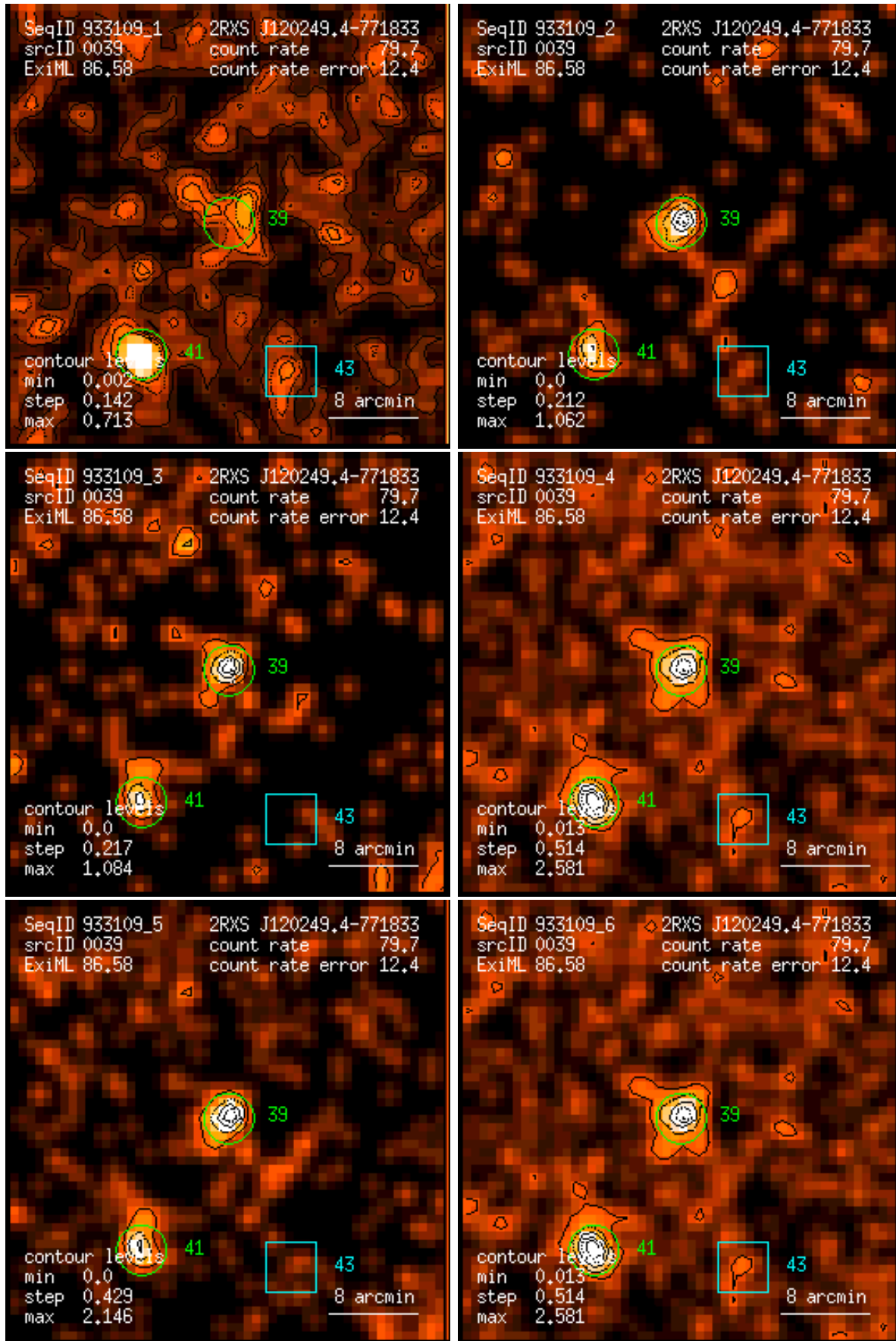
Figure 39: RASS 933109: detection 0039: band rate images, Gaussian filter: (1) PSPC channels 11 – 41, (2) 52 – 90, (3) 91 – 201, (4) 11 – 235, (5) 52 – 201, (6) 11 – 201. Broad band rates in counts/ks. Band rate contour levels in counts/ks/arcmin 2 .
