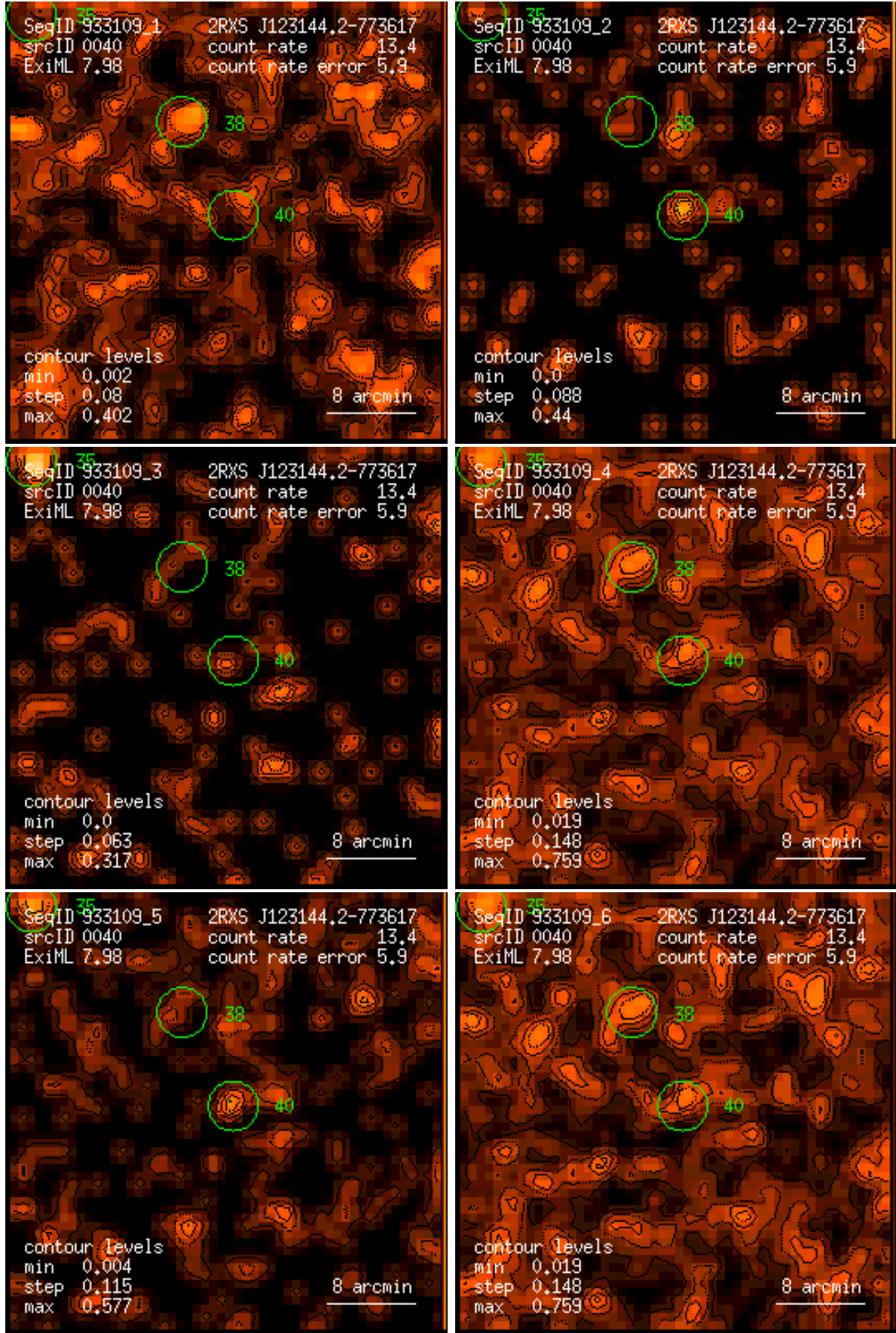
Figure 40: RASS 933109: detection 0040: band rate images, Gaussian filter: (1) PSPC channels 11 – 41, (2) 52 – 90, (3) 91 – 201, (4) 11 – 235, (5) 52 – 201, (6) 11 – 201. Broad band rates in counts/ks. Band rate contour levels in counts/ks/arcmin 2 .
