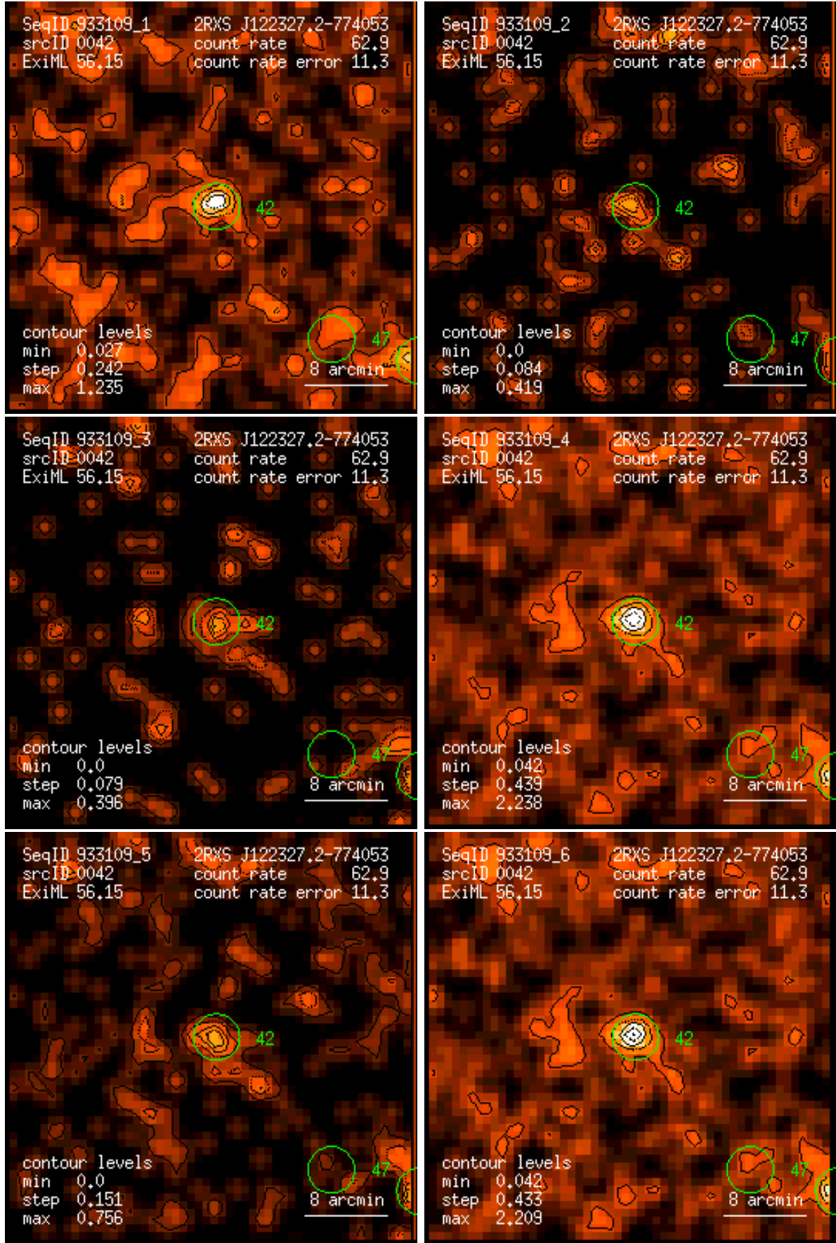
Figure 42: RASS 933109: detection 0042: band rate images, Gaussian filter: (1) PSPC channels 11 – 41, (2) 52 – 90, (3) 91 – 201, (4) 11 – 235, (5) 52 – 201, (6) 11 – 201. Broad band rates in counts/ks. Band rate contour levels in counts/ks/arcmin 2 .
