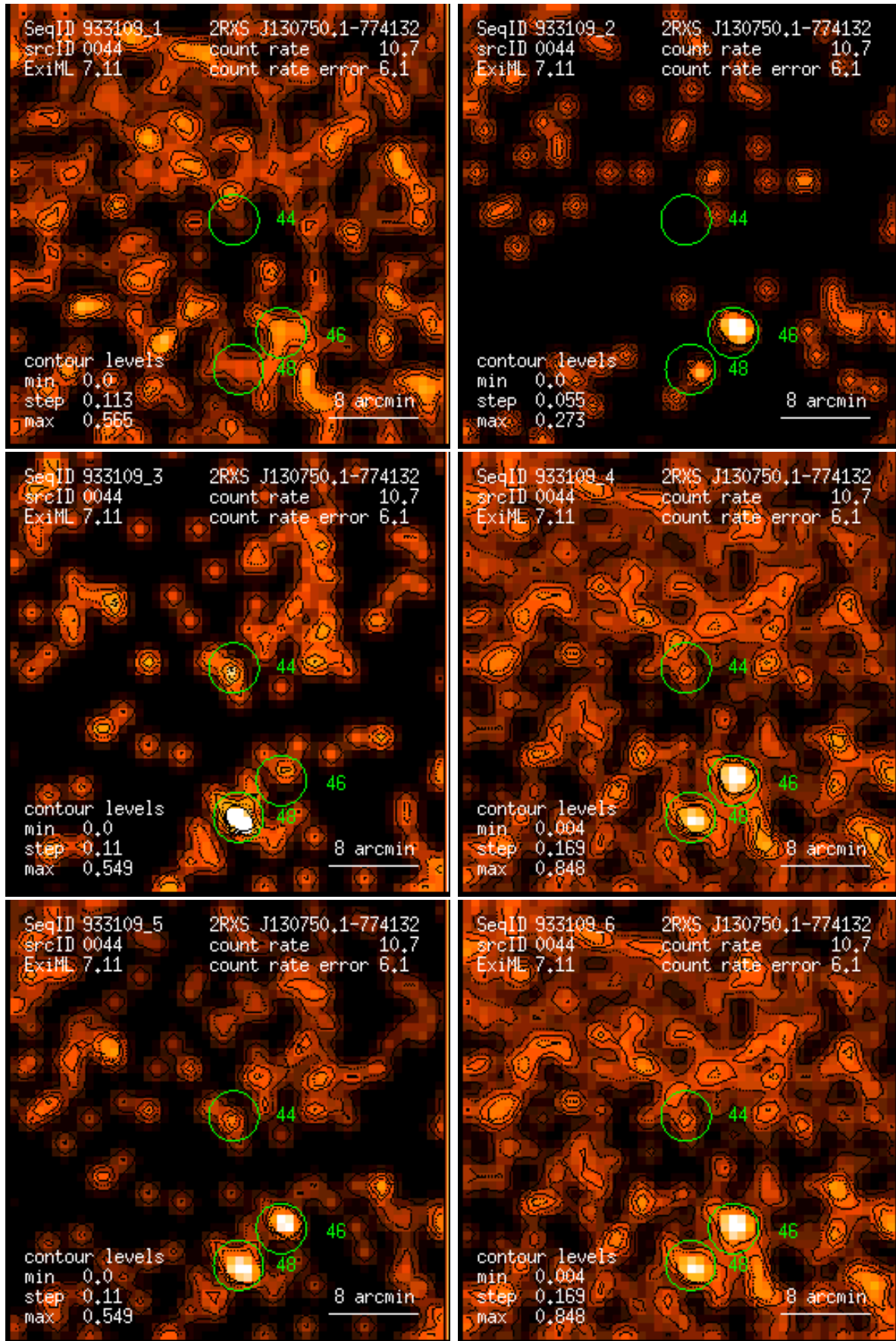
Figure 44: RASS 933109: detection 0044: band rate images, Gaussian filter: (1) PSPC channels 11 – 41, (2) 52 – 90, (3) 91 – 201, (4) 11 – 235, (5) 52 – 201, (6) 11 – 201. Broad band rates in counts/ks. Band rate contour levels in counts/ks/arcmin 2 .
