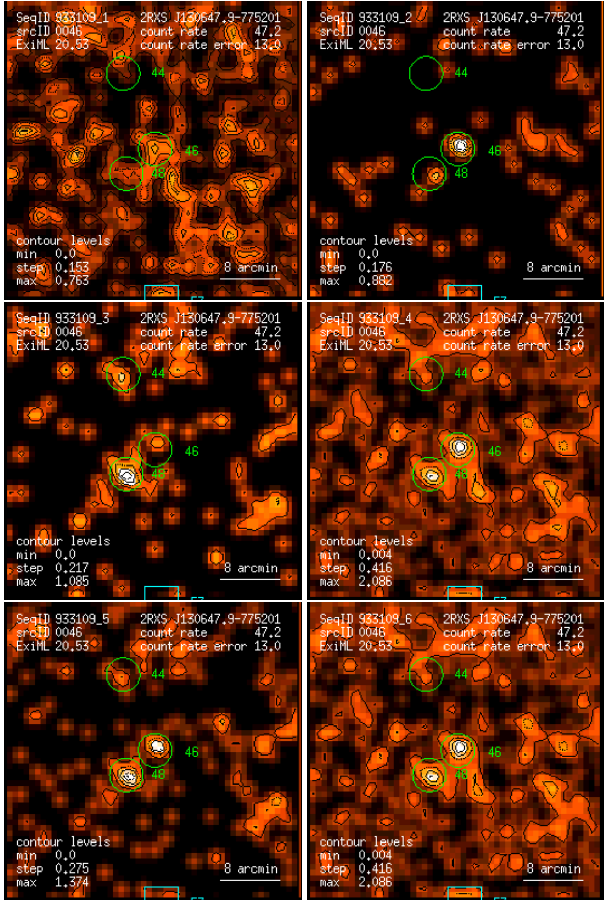
Figure 46: RASS 933109: detection 0046: band rate images, Gaussian filter: (1) PSPC channels 11 – 41, (2) 52 – 90, (3) 91 – 201, (4) 11 – 235, (5) 52 – 201, (6) 11 – 201. Broad band rates in counts/ks. Band rate contour levels in counts/ks/arcmin 2 .
