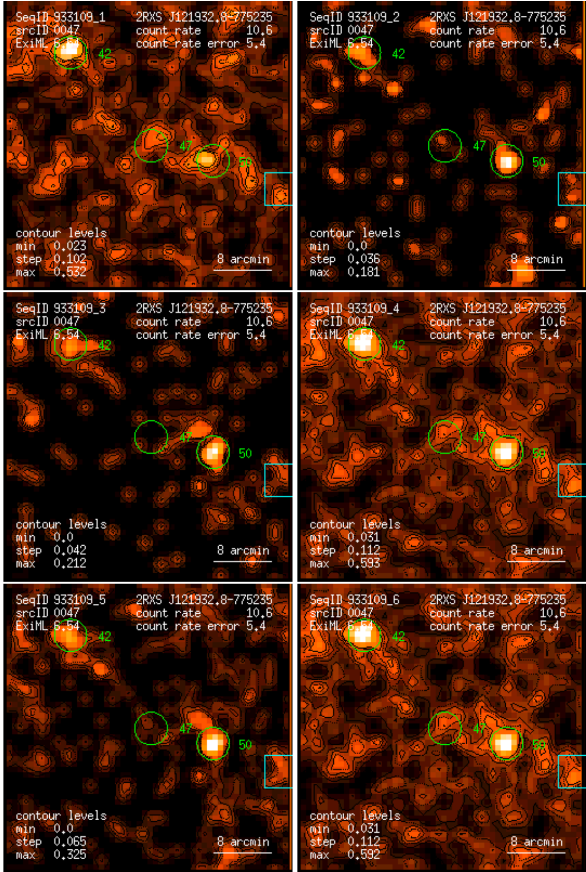
Figure 47: RASS 933109: detection 0047: band rate images, Gaussian filter: (1) PSPC channels 11 – 41, (2) 52 – 90, (3) 91 – 201, (4) 11 – 235, (5) 52 – 201, (6) 11 – 201. Broad band rates in counts/ks. Band rate contour levels in counts/ks/arcmin 2 .
